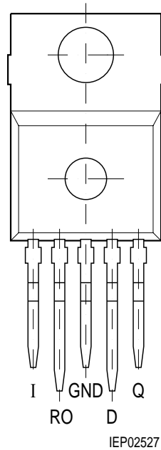
PG-TO220-5-11
