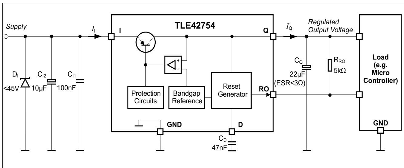
Figure 6 Application diagram
