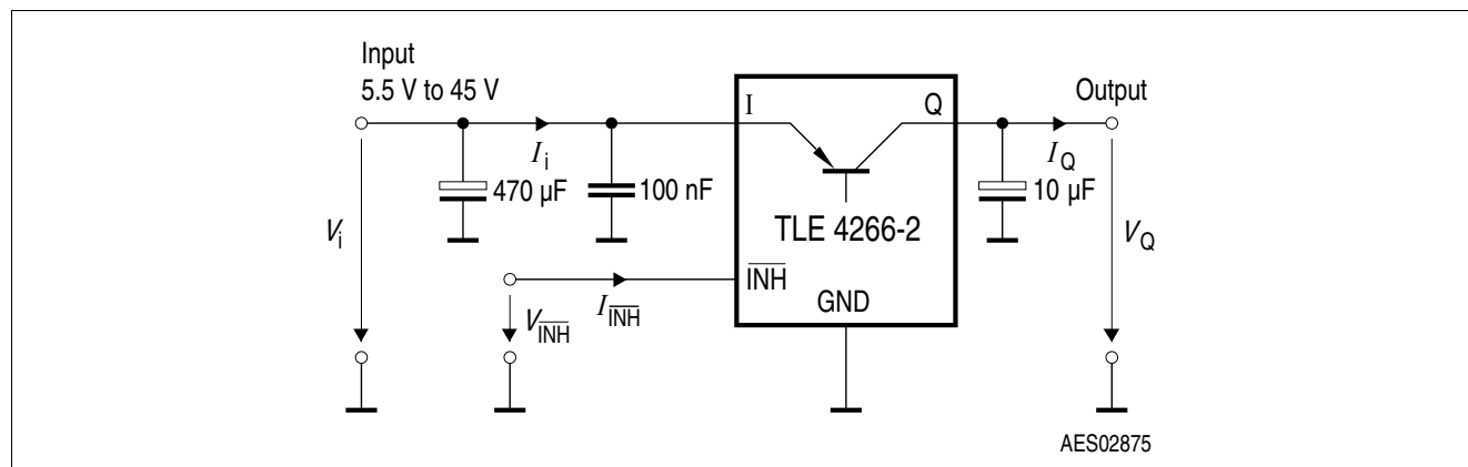
Figure 3 Measuring circuit
