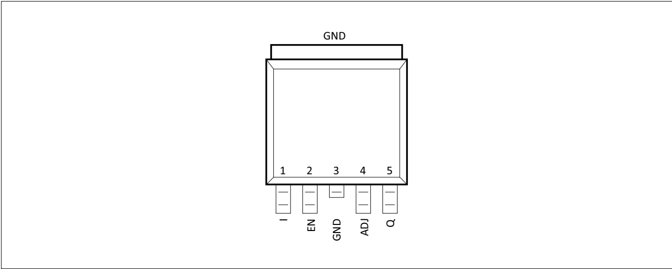
Figure 2 Pin configuration
