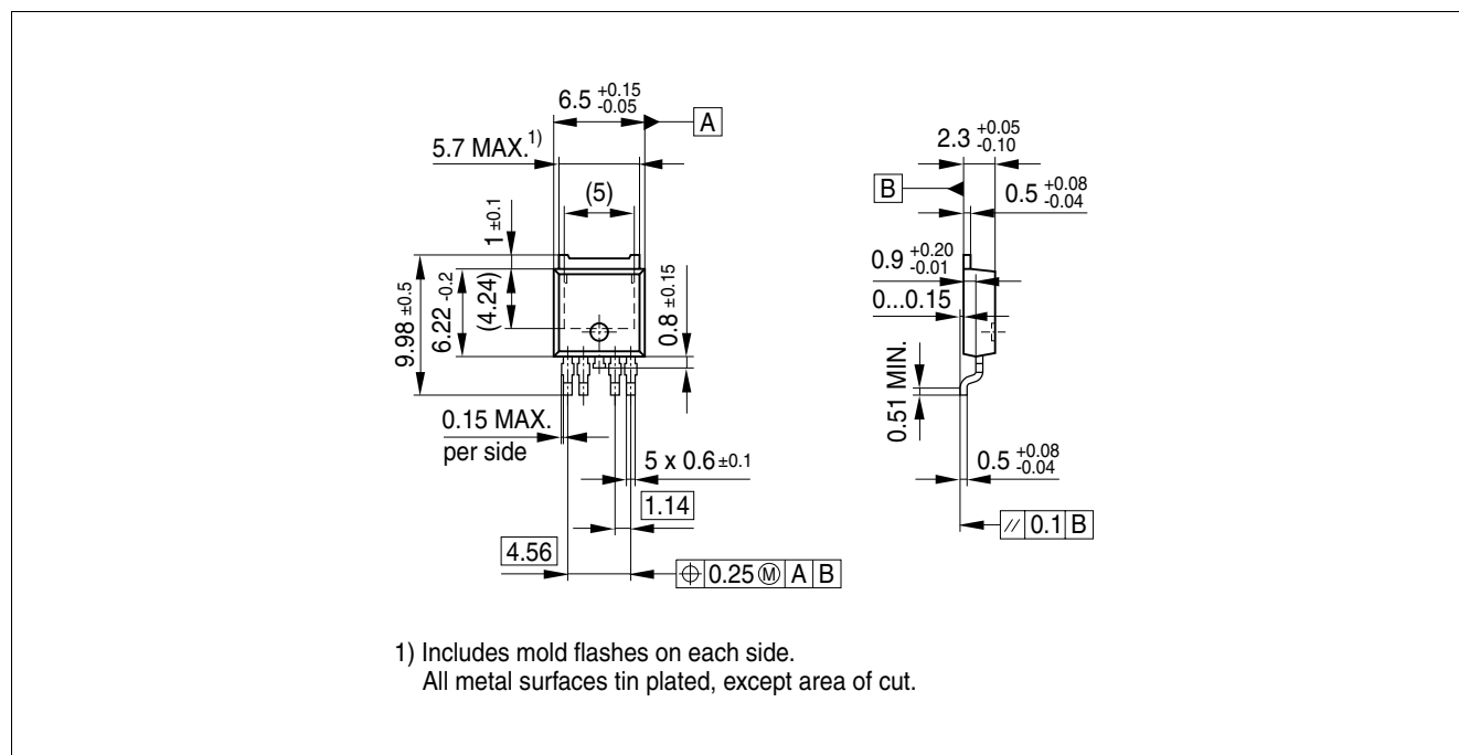
Figure 4 PG-T0252-51 1) (Plastic transistor, single outline)
