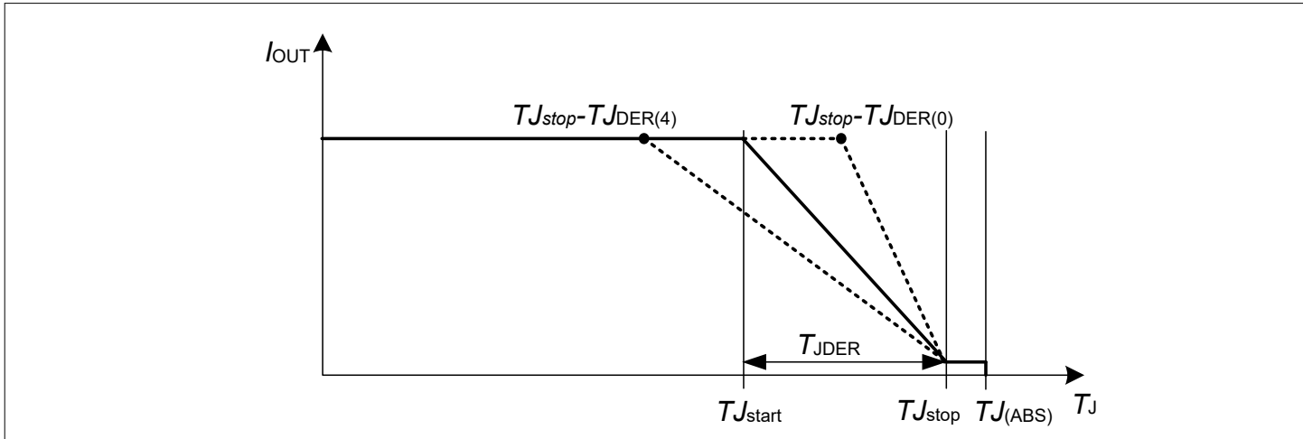
Figure 10 Thermal derating
