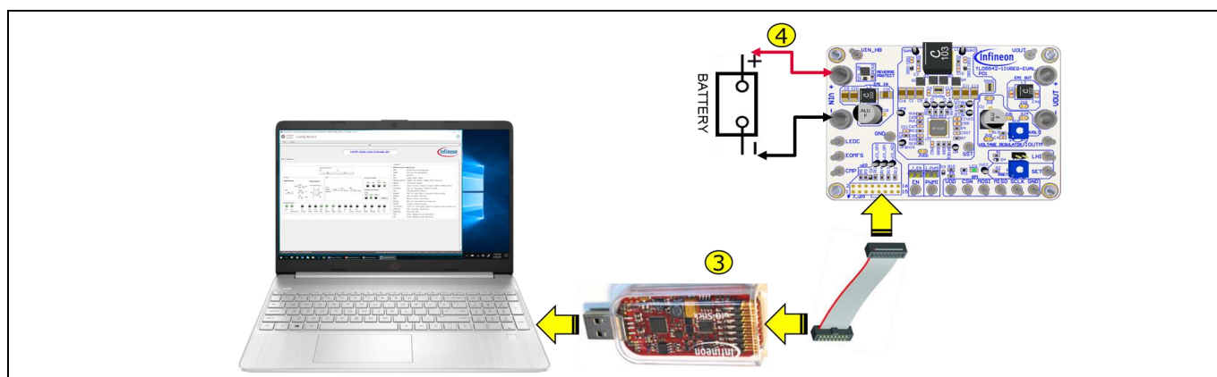
Figure 10 Voltage regulator with \mu IO stick: connect \mu IO and power supply
