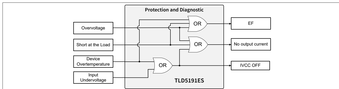
Figure 23 Protection and diagnostic overview - TLD5191ES
