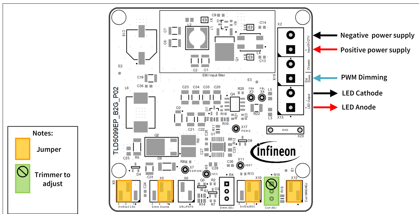
Figure 4 Current adjustment
