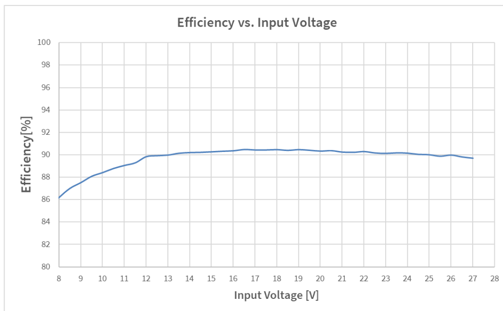
Figure 13 Efficiency vs. input voltage
