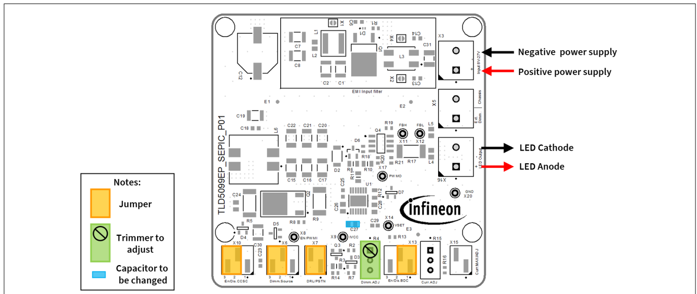
Figure 6 Embedded PWM engine
