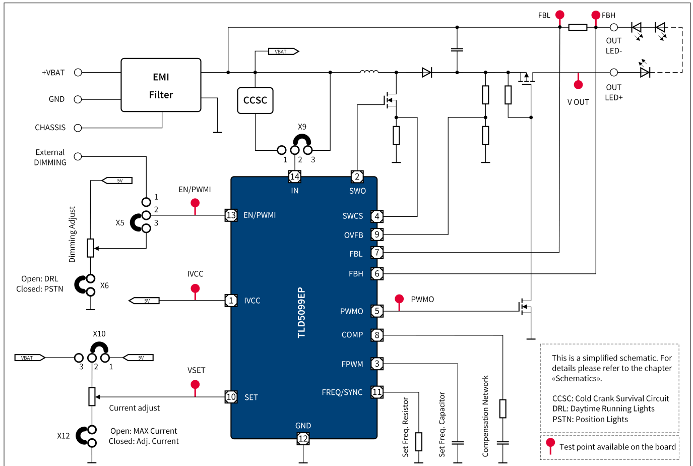
Figure 2 Simplified schematic
