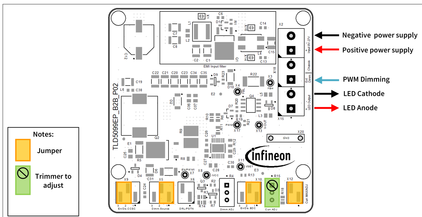
Figure 4 Current adjustment
