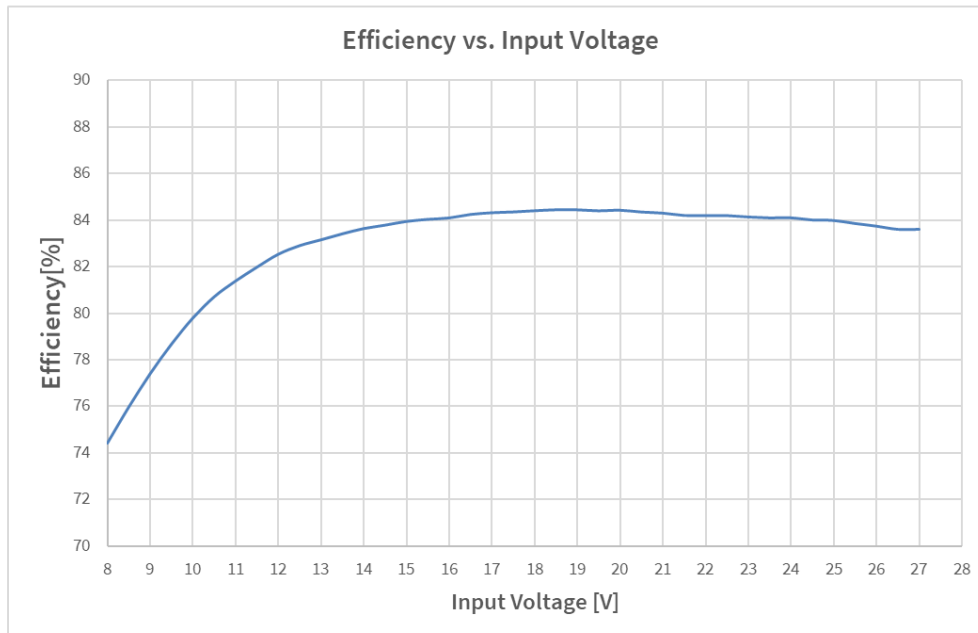
Figure 13 Efficiency vs. input voltage
