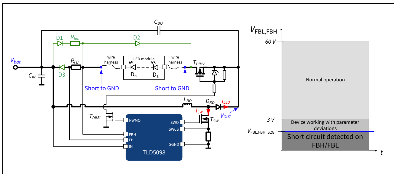
Figure 16 Short circuit to GND protection
