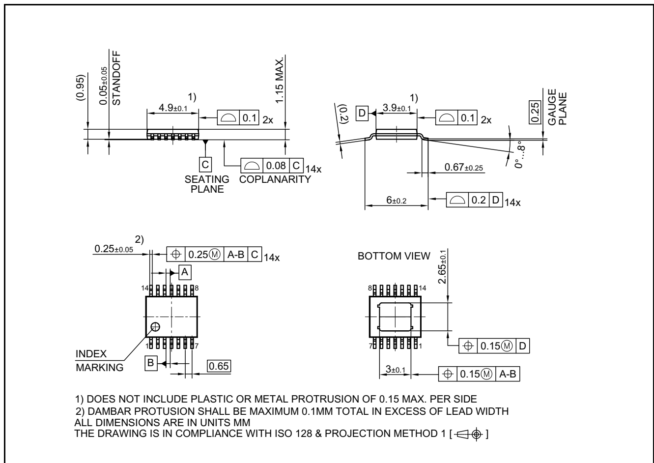
Figure 31 Outline PG-TSDSO-14 1)
