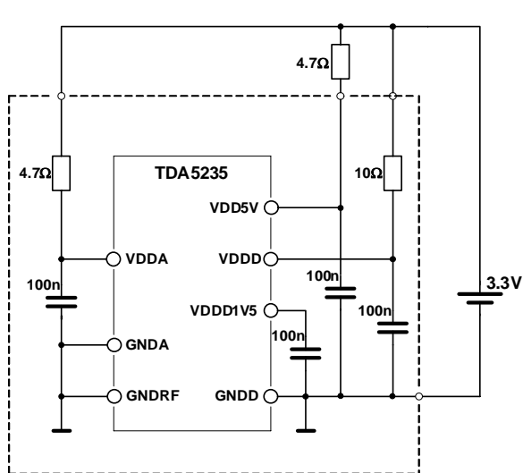
Supply-Application in 3.3V environment
