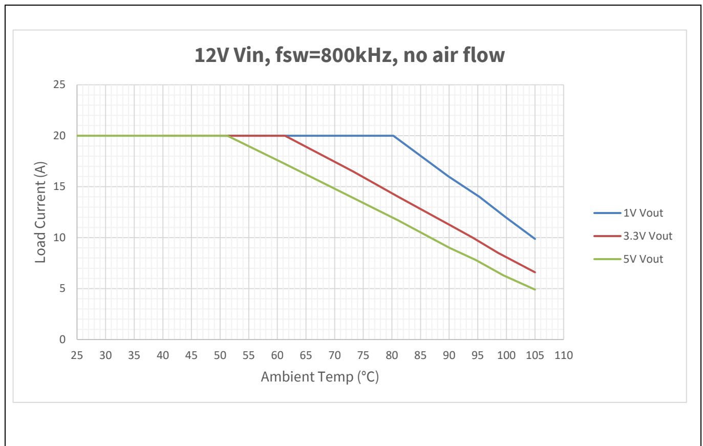
Figure 5 Thermal de-rating
