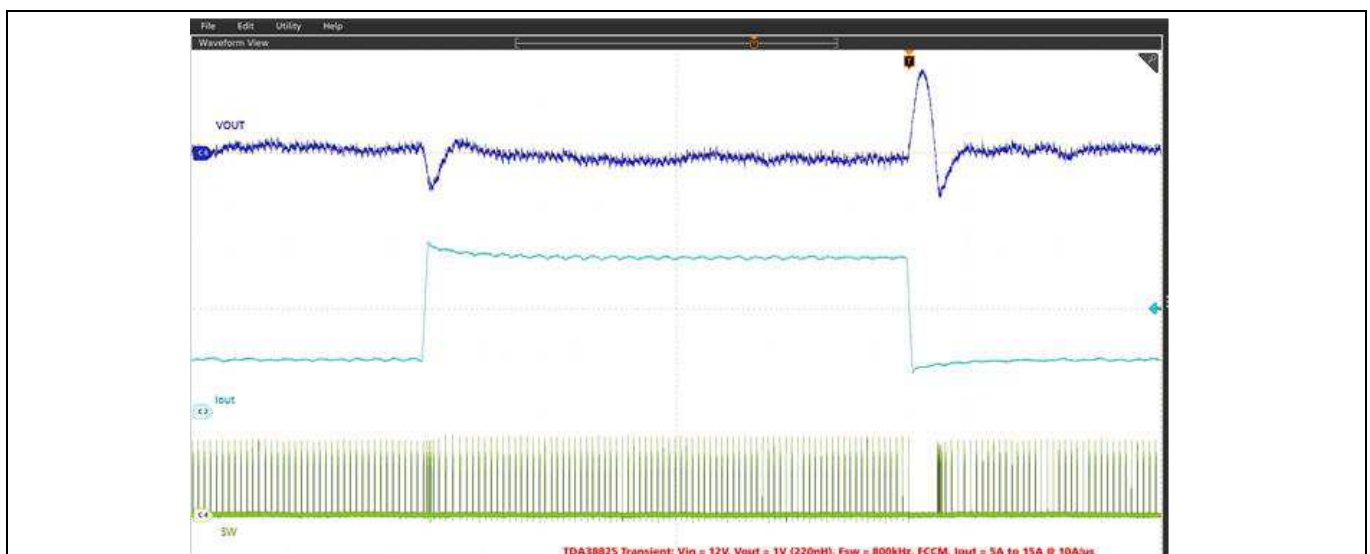
Figure 20 Transient response at 10 A step load current @ 10 A/μs slew rate: I_o = 5\text{ A} - 15\text{ A} , (Ch6: Vo, Ch2: Io, Ch4: SW), pk-pk: 39.4 mV, Fsw = 800 kHz
