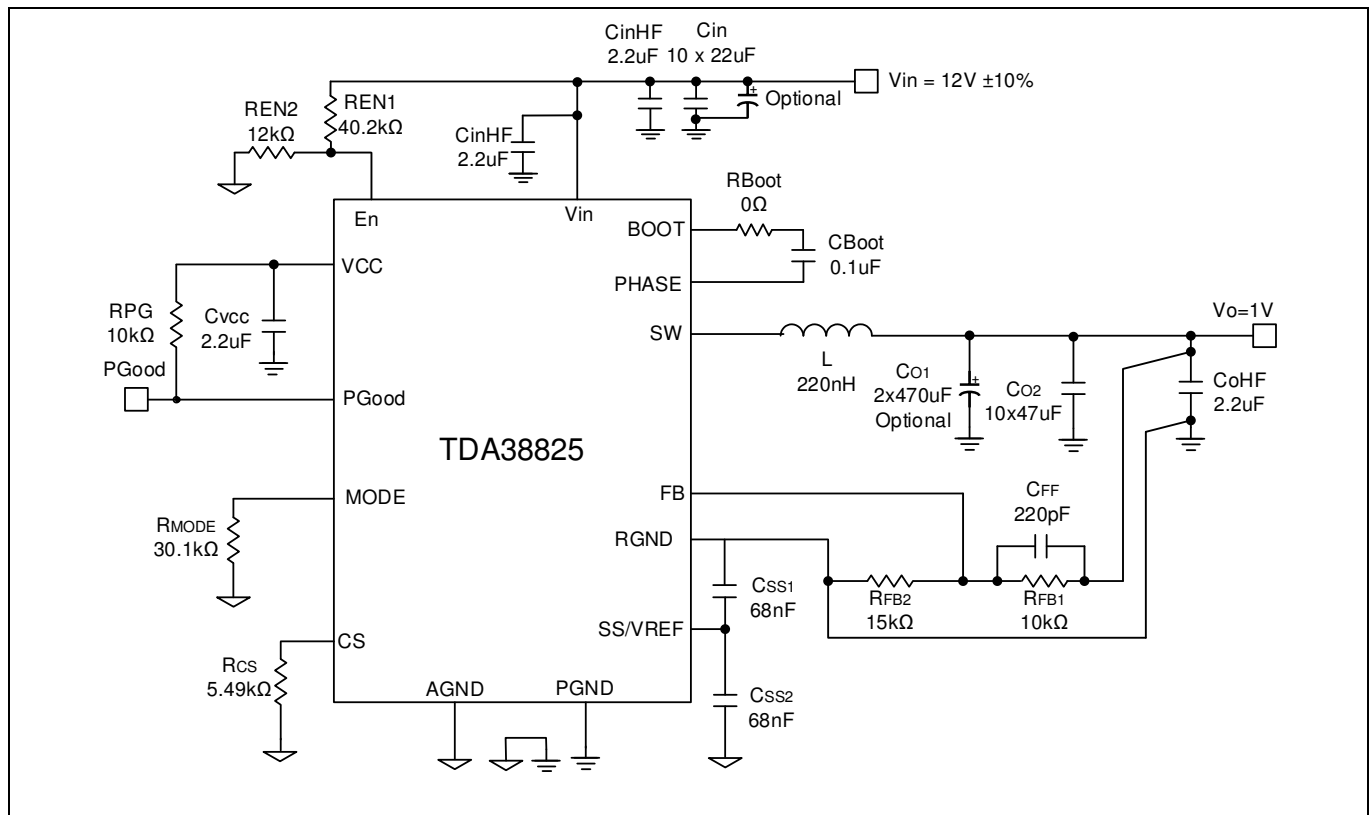
Figure 13 Typical application diagram of TDA38825. V_{in} = 12V , V_o = 1V , I_o = 20A , F_{sw} = 800kHz .
