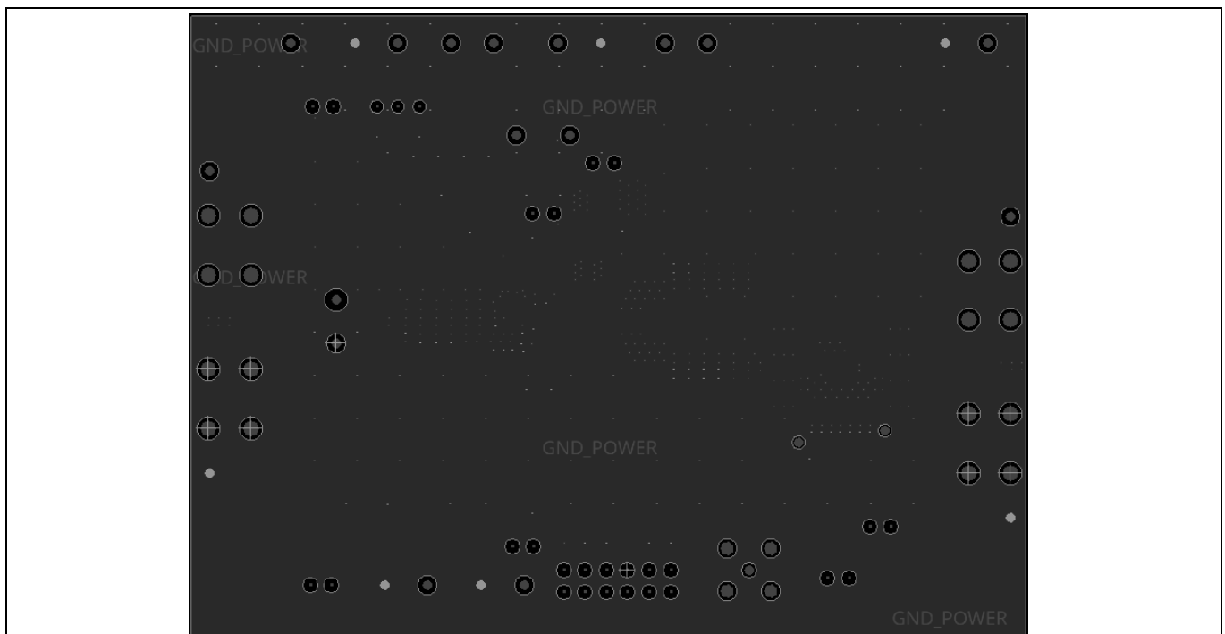
Figure 26 TDA38825 Demo Board – 5th Layer (Ground)
