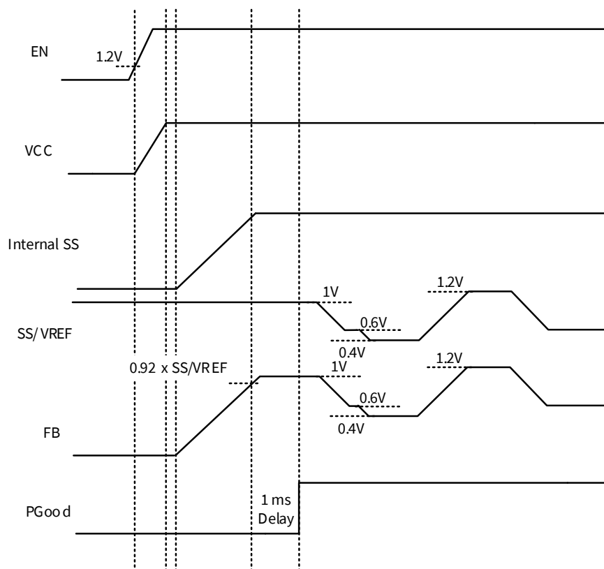
(a) Startup sequence with external reference
