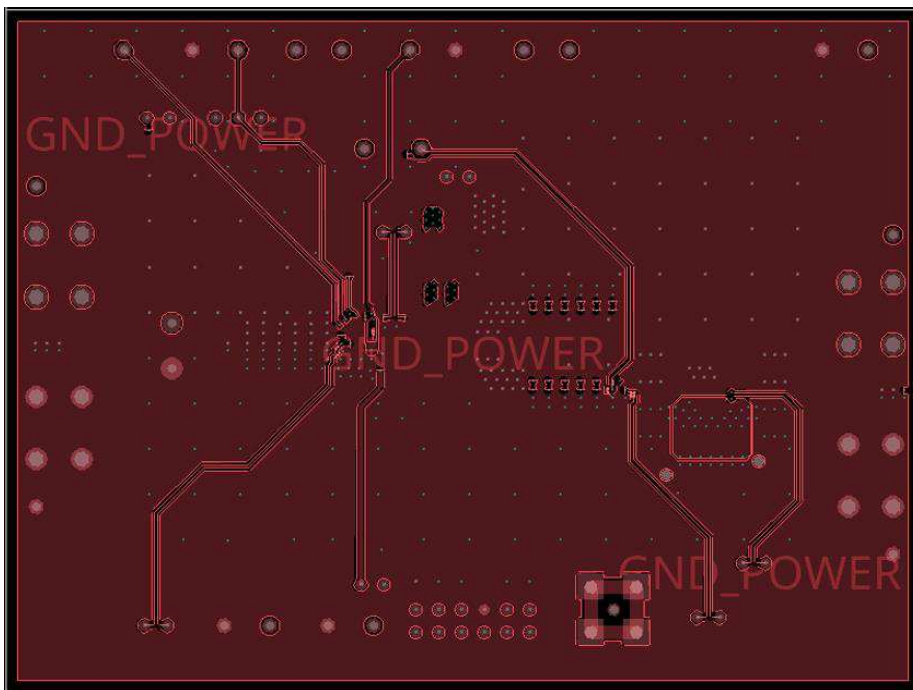
Figure 24 TDA38813 Demo Board – 3rd Layer (Ground & Signal)
