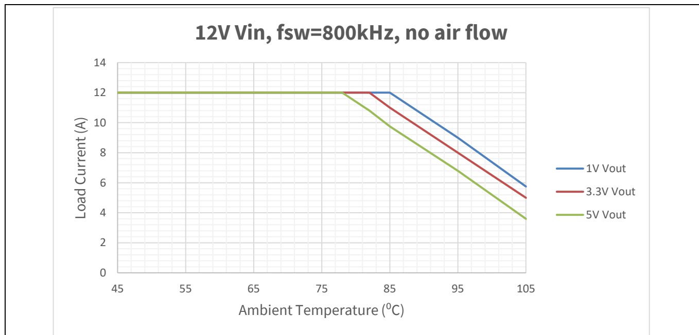
Figure 5 Thermal Derating
