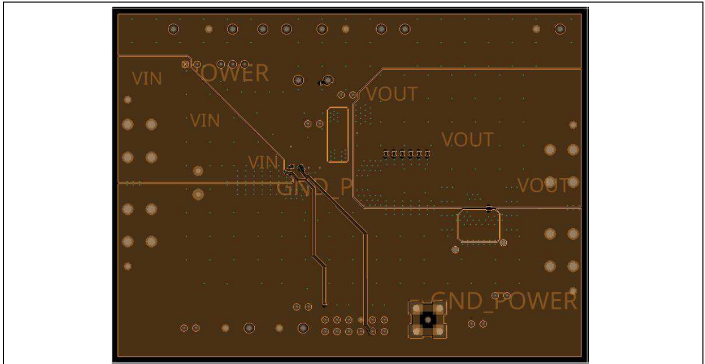
Figure 25 TDA38813 Demo Board – 4th Layer (Ground & Signal)
