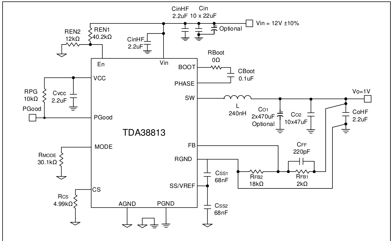
Figure 13 Typical application diagram of TDA38813. V_{in} = 12V , V_o = 1V , I_o = 12A , F_{sw} = 800kHz .
