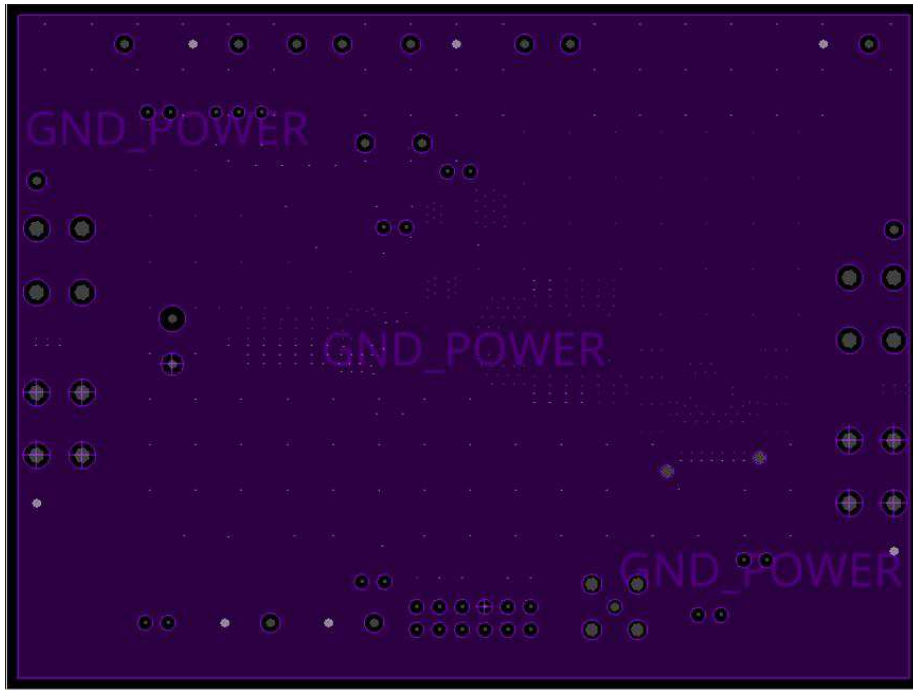
Figure 23 TDA38813 Demo Board – 2nd Layer (Ground)
