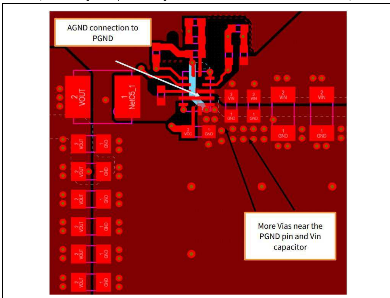
Figure 9 Layout Diagram
