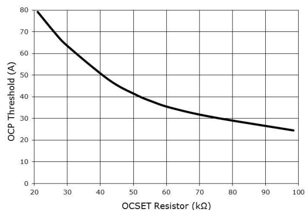
Figure 8 Programmable OCP Threshold
