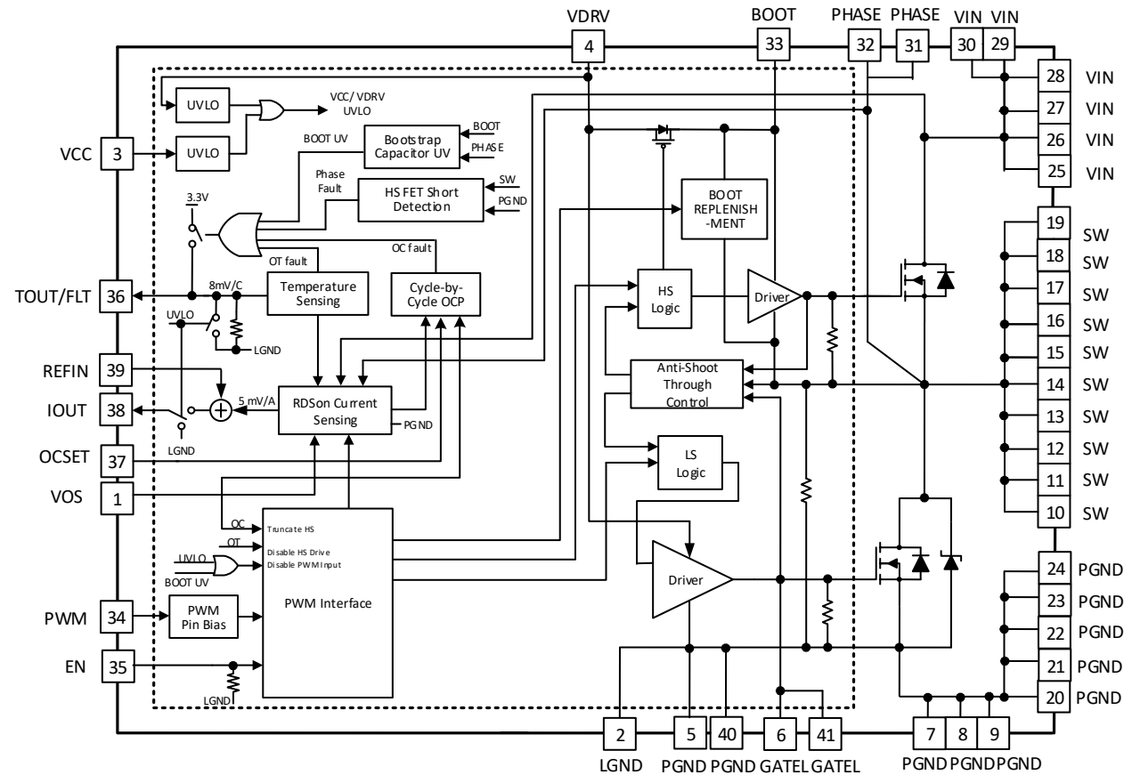
Figure 3 Block Diagram
