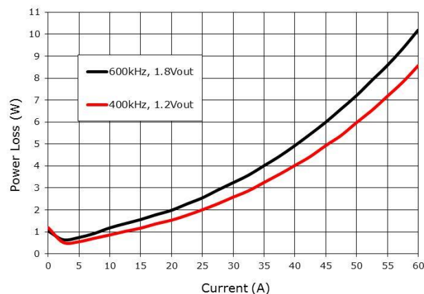
Figure 7 Power Stage Loss
