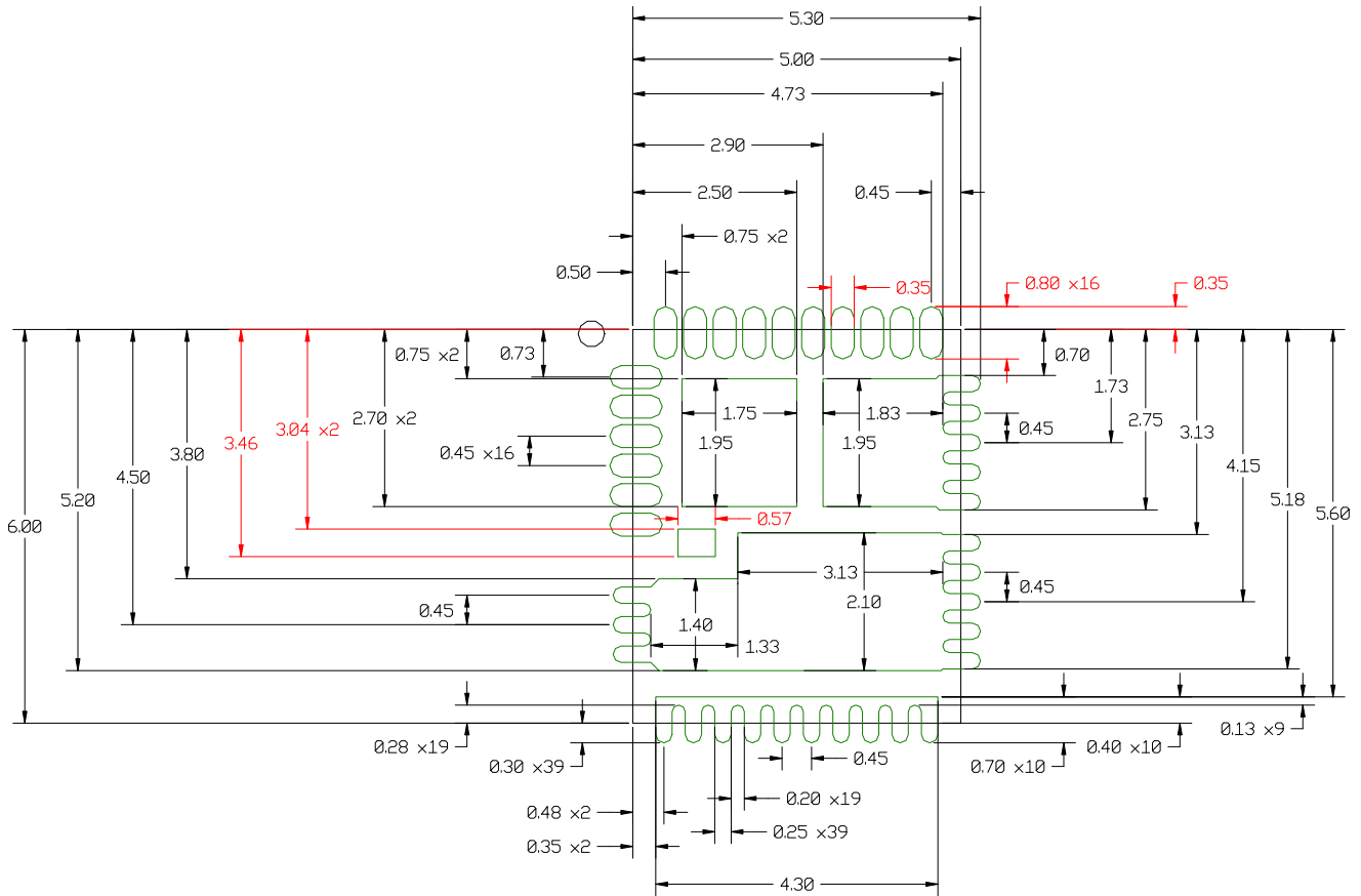
Figure 16 Solder Resist
