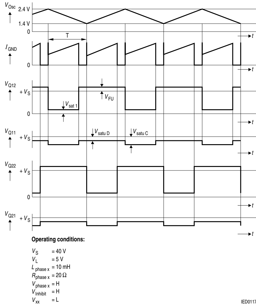
Figure 9 Current Control
