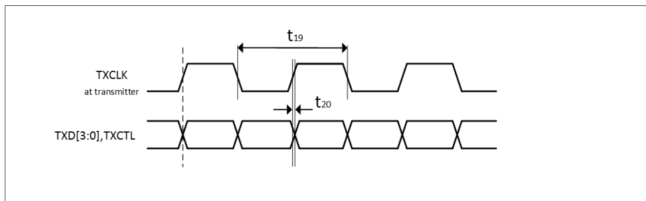
Figure 3-20 ETH RGMII TX Signal Timing (Delay on Destination (DoD))
