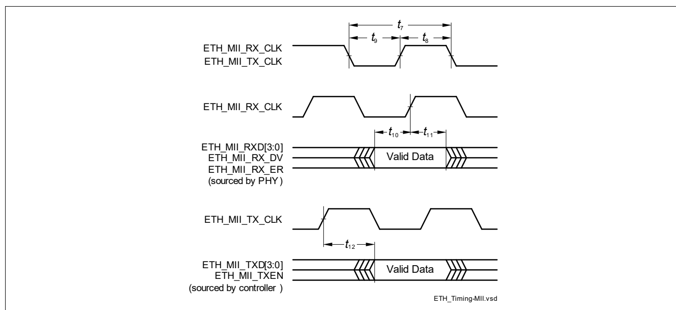
Figure 3-18 ETH MII Signal Timing
