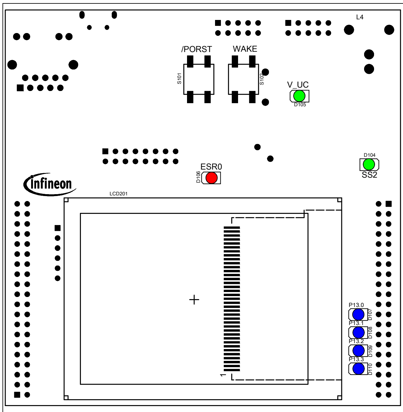
Figure 2-3 Application Kit TC2X7 V1.X Bottom Placement
