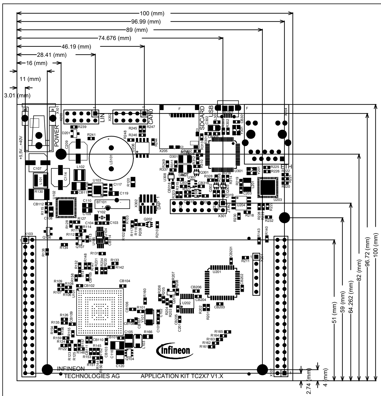
Figure 6-7 Dimensioning (mm)
