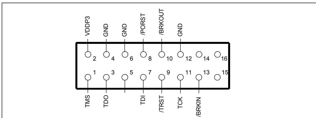
Figure 5-7 OCDS connector pinout (IDC16)
