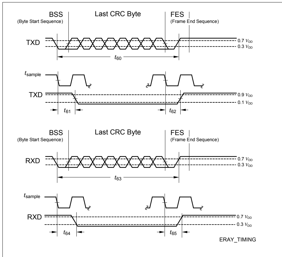
Figure 25 ERAY Timing
