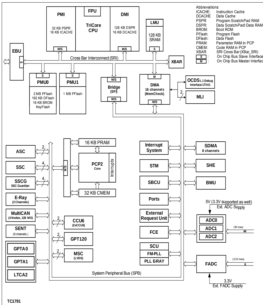
Figure 4 Block Diagram
