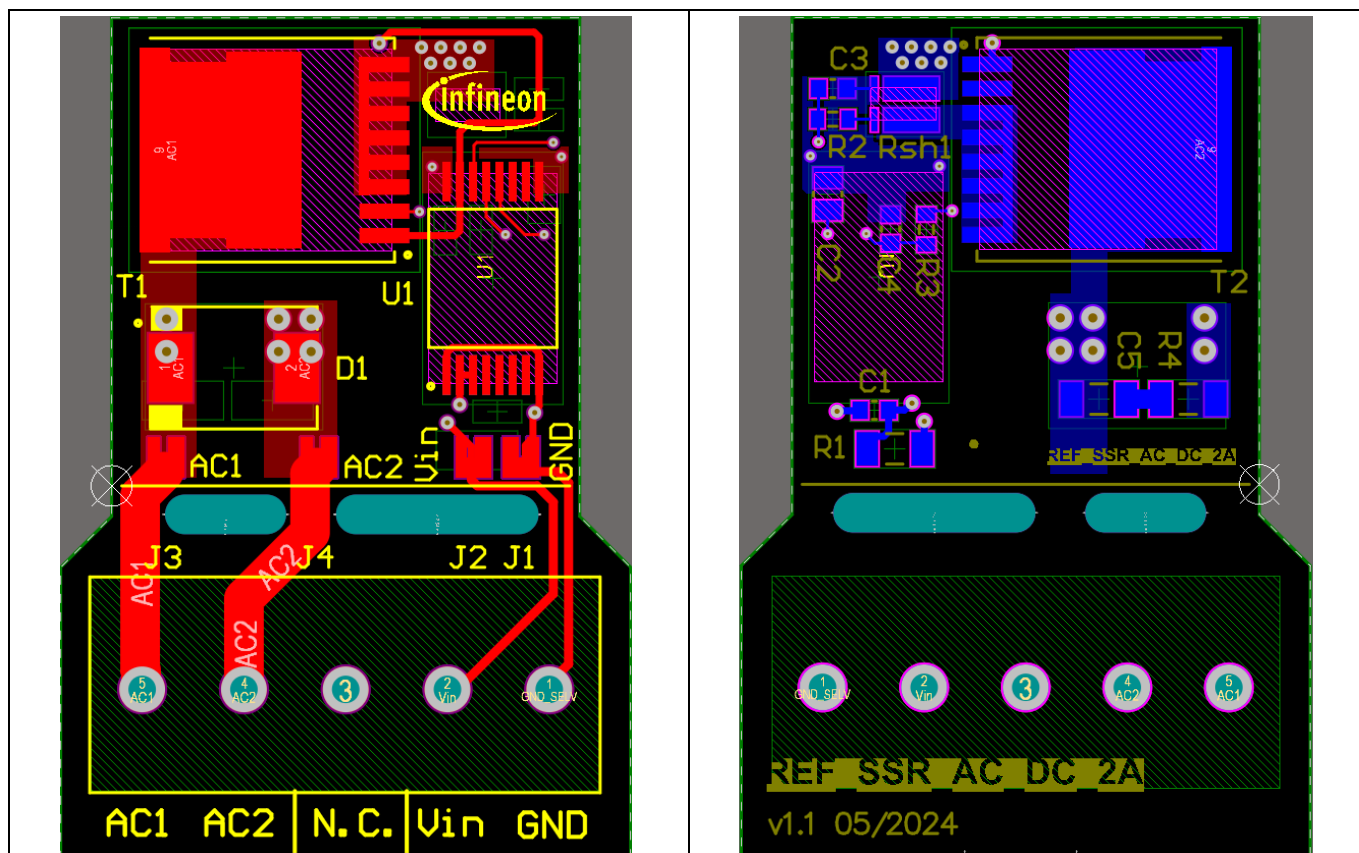
Figure 7 Top (left) and bottom (right) layers of REF_SSR_AC_DC_2A
