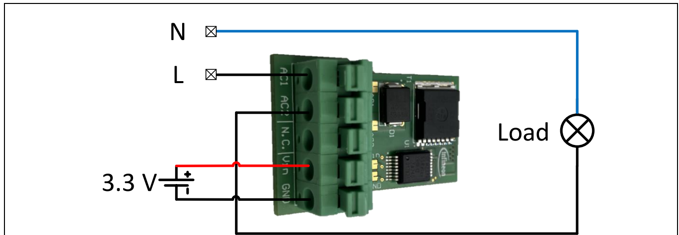
Figure 3 SSR connection diagram
