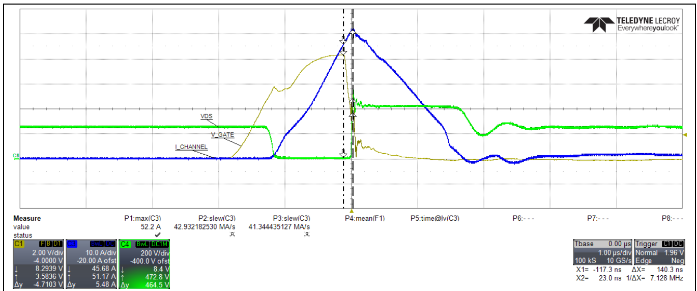
Figure 10 Short-circuit event
