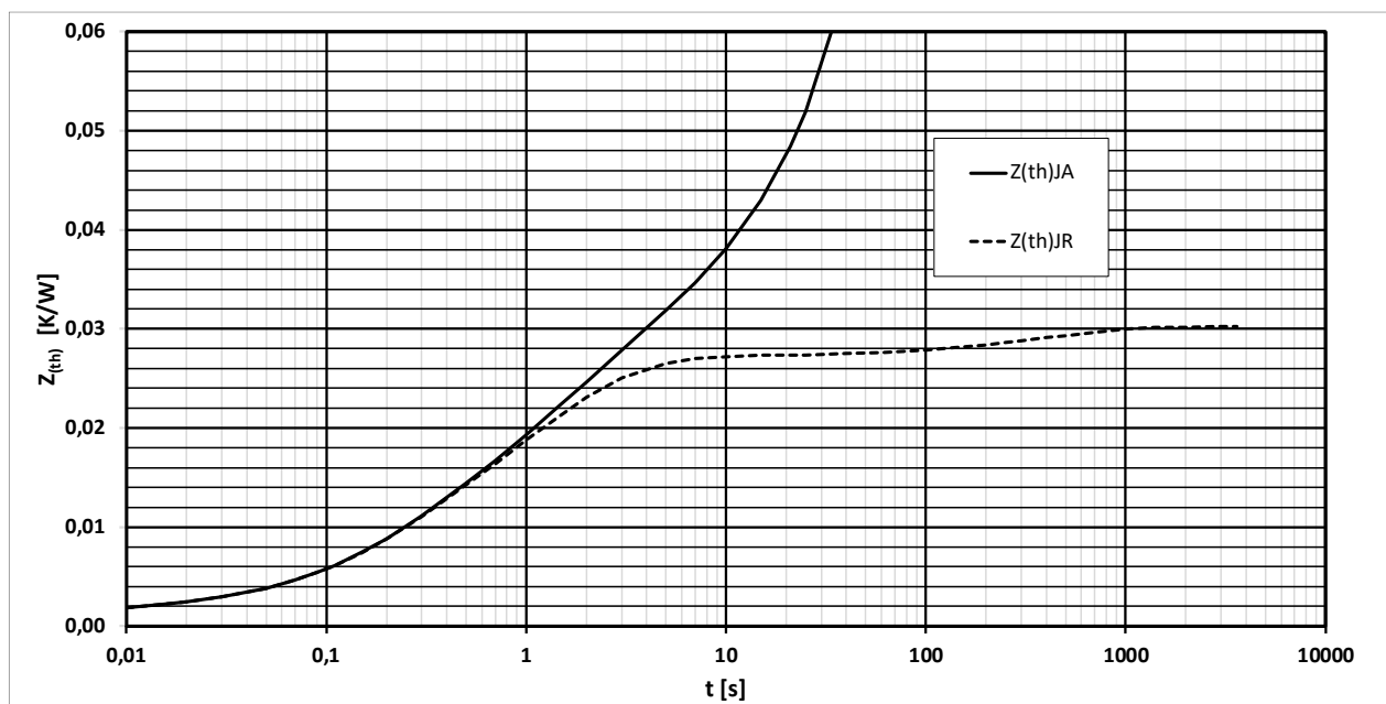
Transienter Wärmewiderstand je Zweig / Transient thermal impedance per arm Z_{thJR} = f(t) ; Z_{thJA} = f(t)
