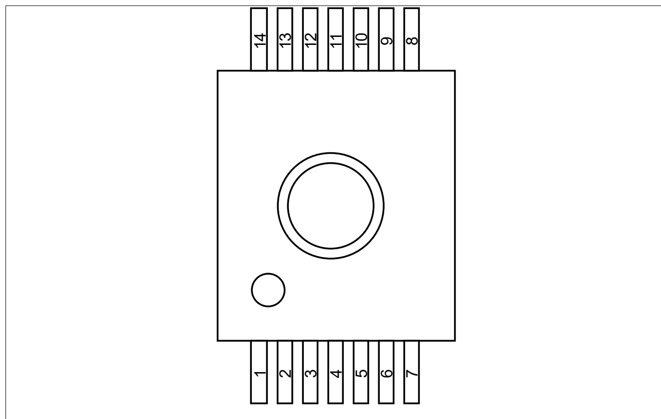
Figure 2 Pin Configuration
