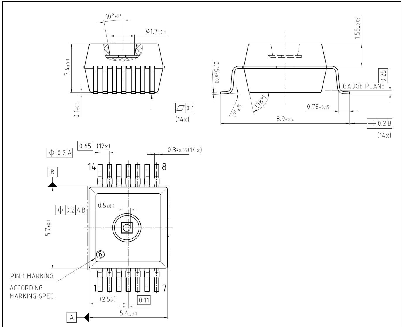
Figure 8-1 Package Outline
