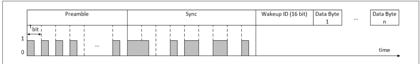
Figure 18 LF telegram modulated on a 125 kHz carrier (shaded areas)
