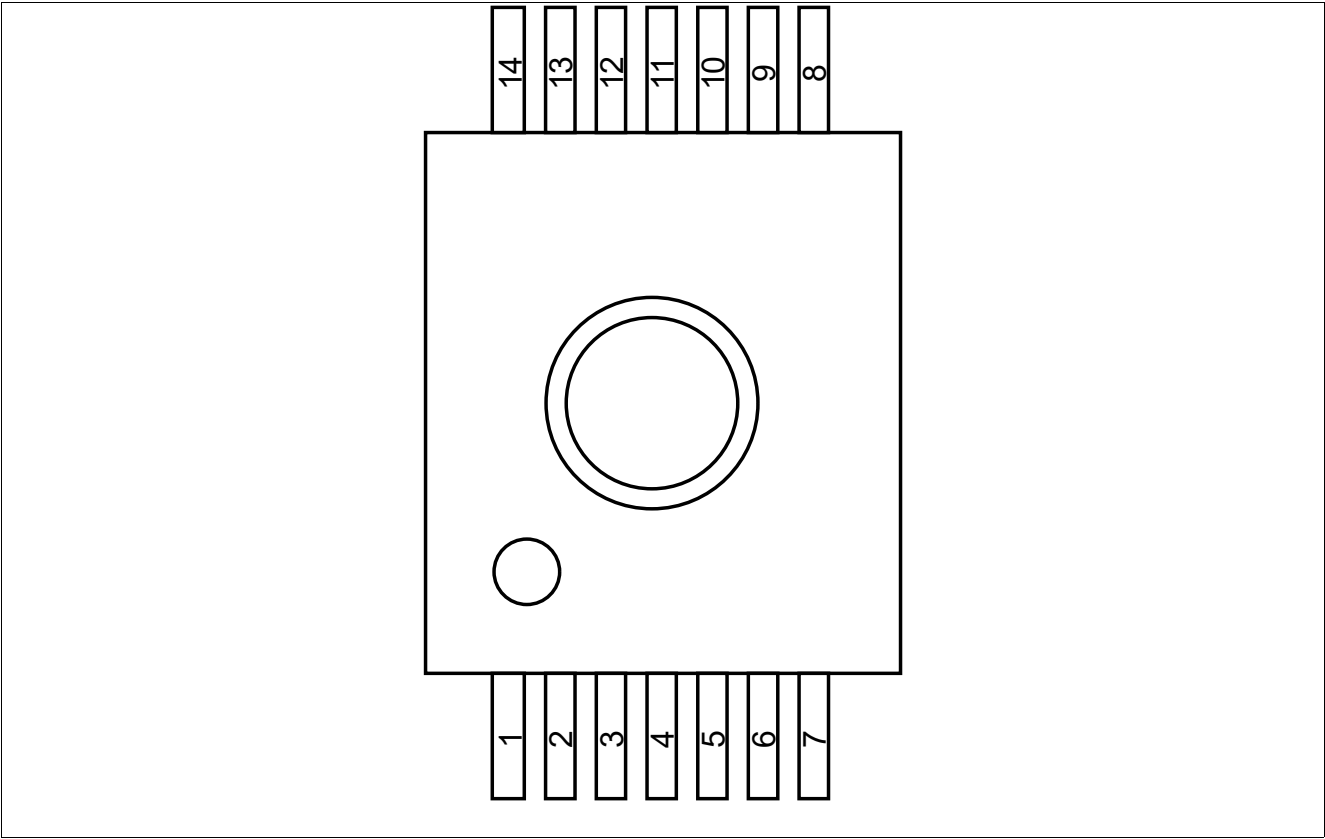
Figure 1 Pin Configuration
