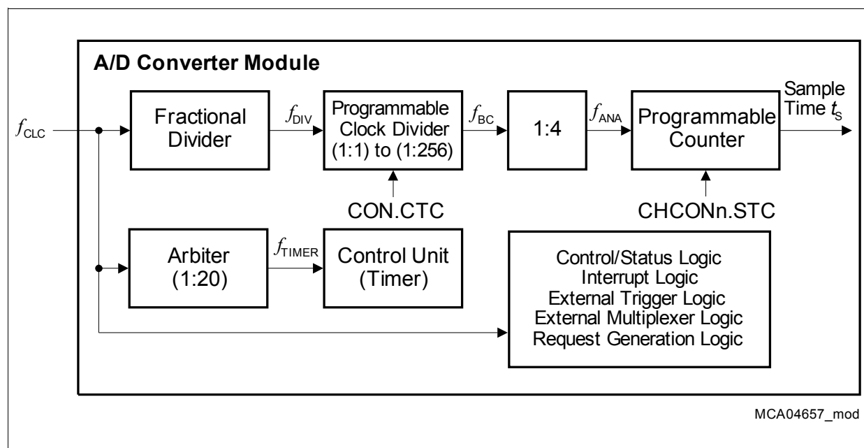
Figure 22 ADC0/ADC1 Clock Circuit
