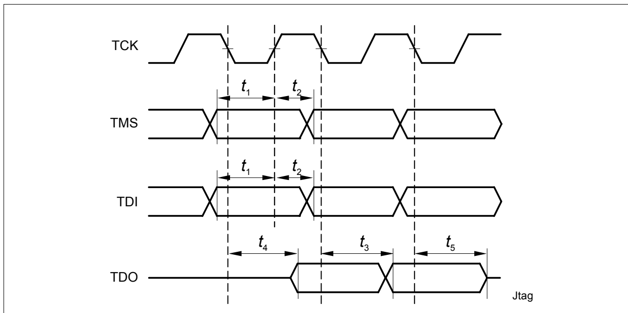
Figure 37 JTAG Timing
