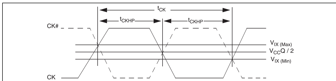
Figure 28 Clock characteristics
