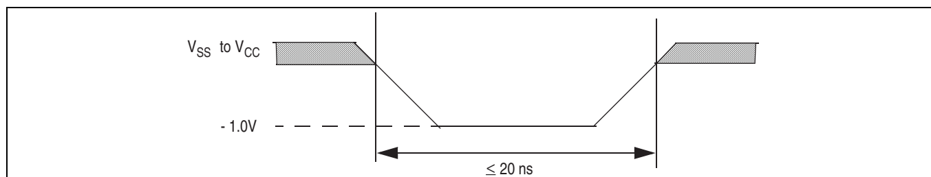
Figure 14 Maximum negative overshoot waveform
