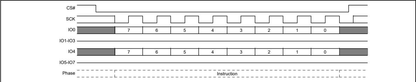
Figure 52 Write Disable (WRDI) command sequence
