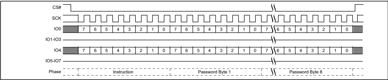
Figure 100 Password Program command sequence
