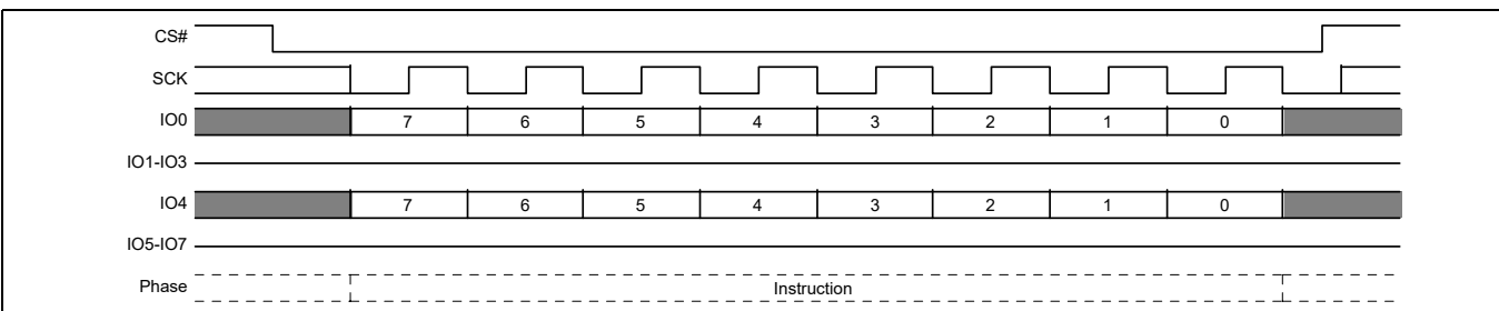
Figure 108 Release from Deep Power-Down command sequence
