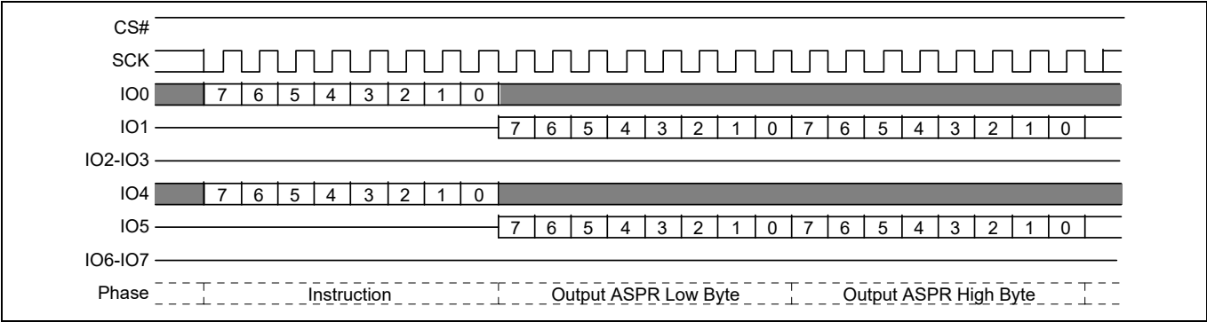
Figure 88 ASPRD command
