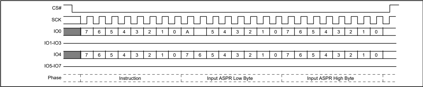
Figure 89 ASPP command
