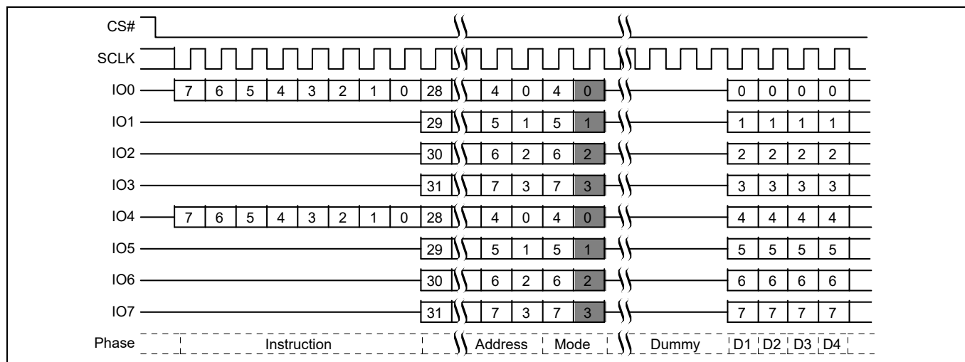
Figure 10 Dual-Quad, Quad I/O command [4, 5]
