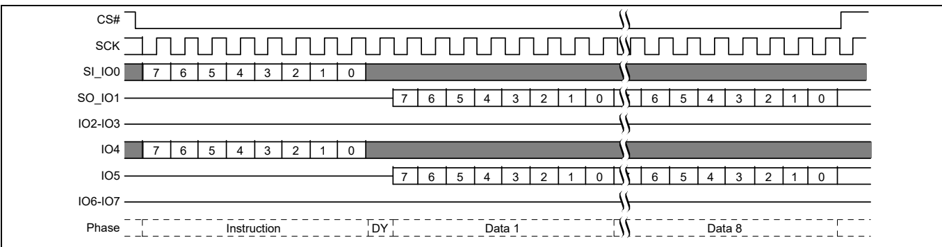
Figure 99 Password Read command sequence
