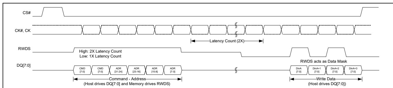
Figure 11 WRITE with 2X latency transaction (DDR) [18, 19, 20]
