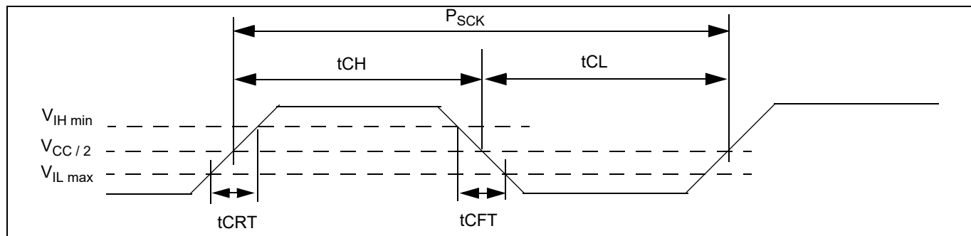
Figure 28 Clock timing
