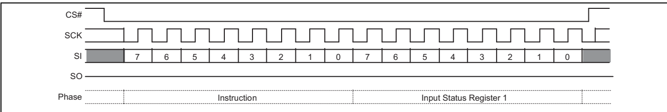
Figure 59 Write Registers (WRR) command sequence – 8-data bits
