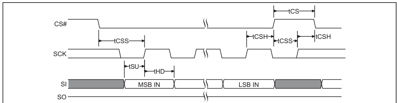
Figure 29 SPI single bit input timing
