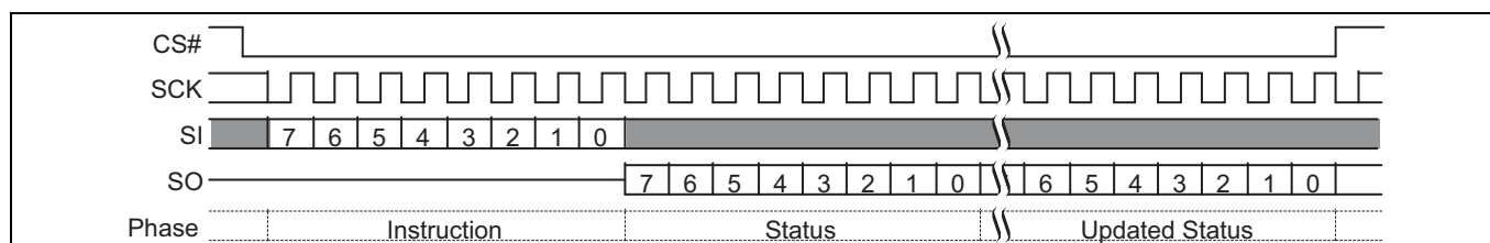
Figure 55 Read Status Register 1 (RDSR1) command sequence
