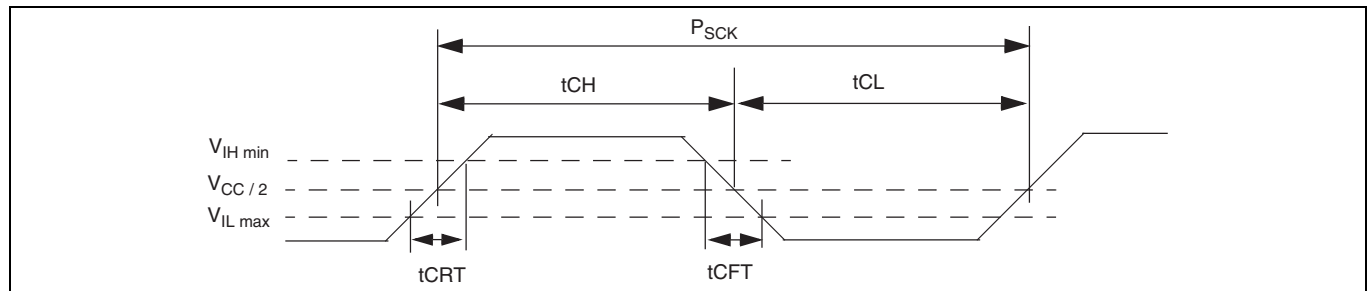
Figure 28 Clock timing
