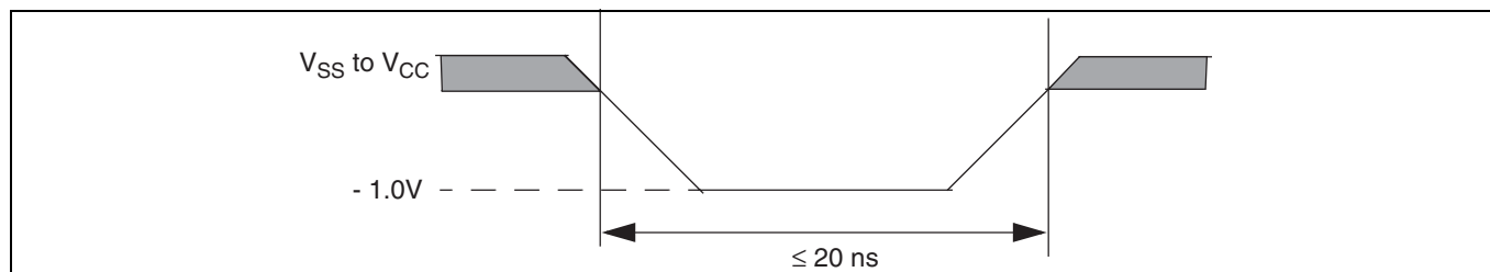
Figure 16 Maximum negative overshoot waveform
