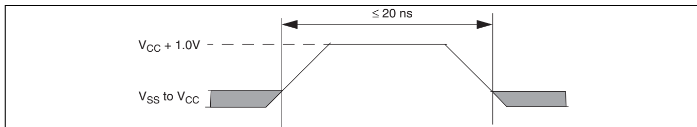
Figure 17 Maximum positive overshoot waveform
