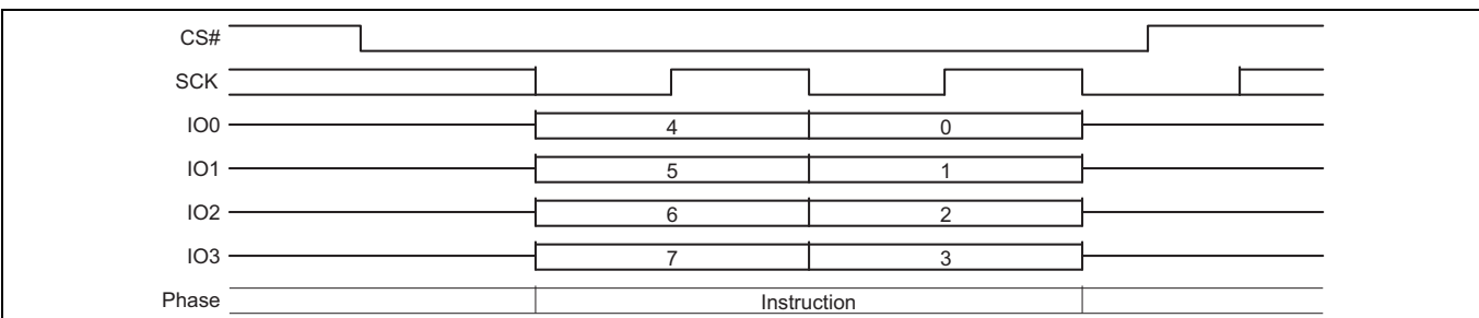
Figure 121 DPD command sequence QPI Mode
