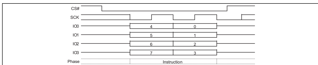
Figure 117 Software Reset command sequence QPI Mode
