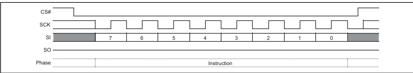
Figure 120 Deep Power-Down command sequence
