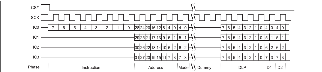
Figure 14 DDR Quad I/O Read
