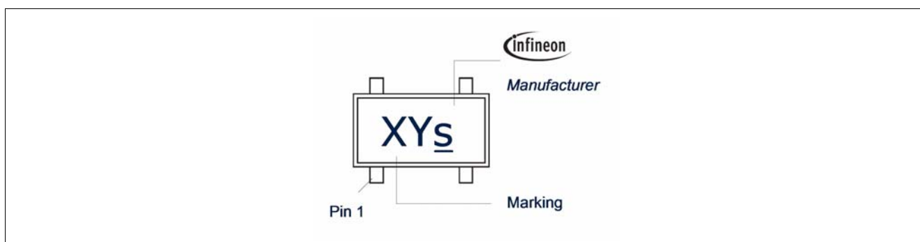
Figure 7-3 Marking Description (Marking BFP640FESD: T4s)
