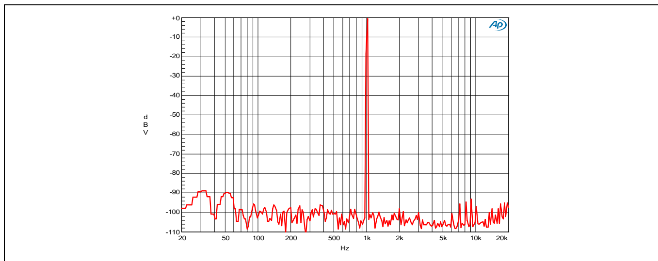
Figure 7 Noise floor with 1 V_{\text{RMS}} output 4 \Omega load
