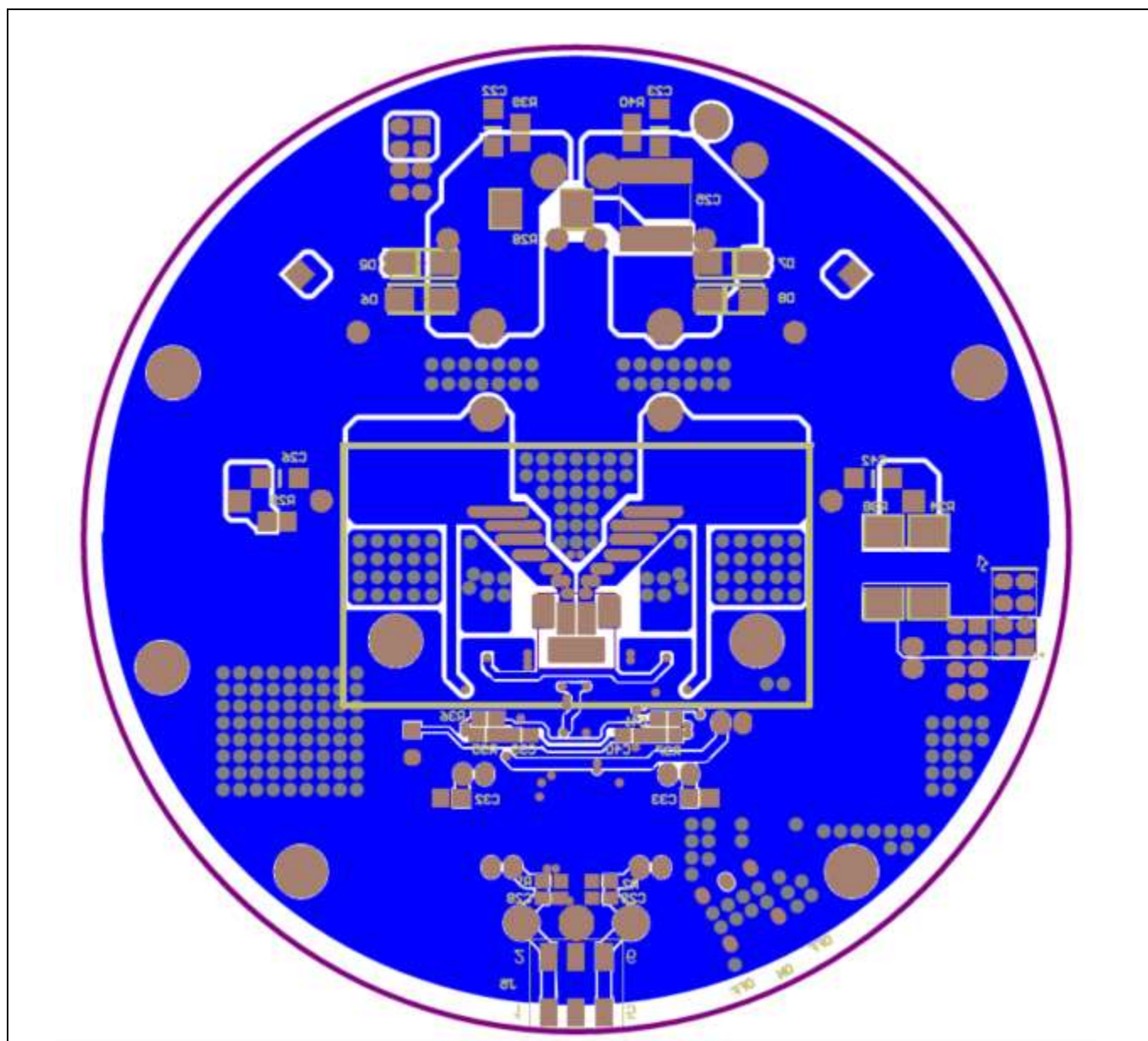
Figure 16 Board bottom view
