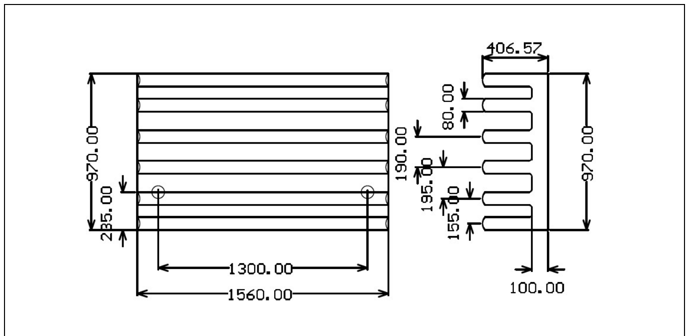
Figure 11 Heatsink dimension
