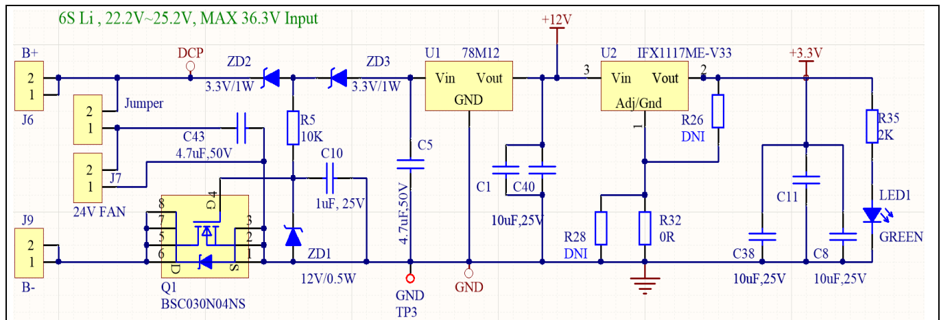
Figure 29 Power supply section of the REF-Vacuum-C101-2ED reference design
