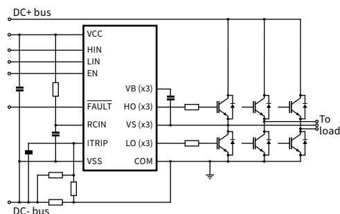
Typical connection
