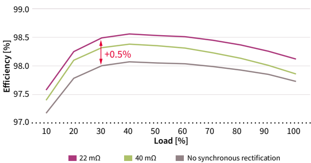
Efficiency in 2400 W PFC at V_{in} = 230 V_{AC} Difference between using or not using the active bridge rectification
