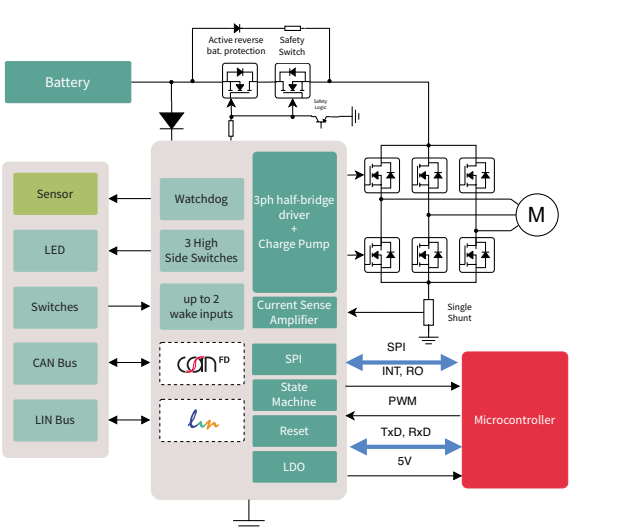
Application diagram TLE9563/4 for BLDC motor control
