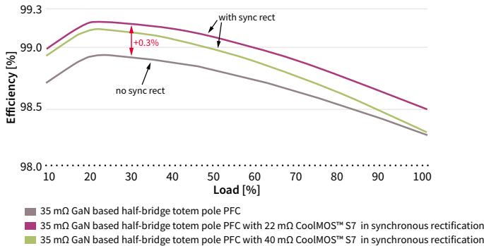
3 kW GaN based totem pole PFC efficiency calculation with and without synchronous rectification when V_{in} = 230 V_{AC} , V_{out} = 400 V , f_{sw} = 65 kHz
