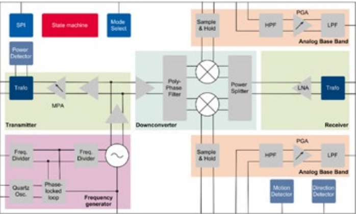
Block diagram of the BGT60LTR11AIP
