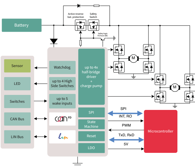
Application diagram TLE9560/1/2 for DC motor control
