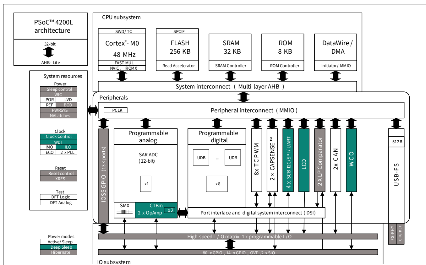
Figure 2 Block diagram
