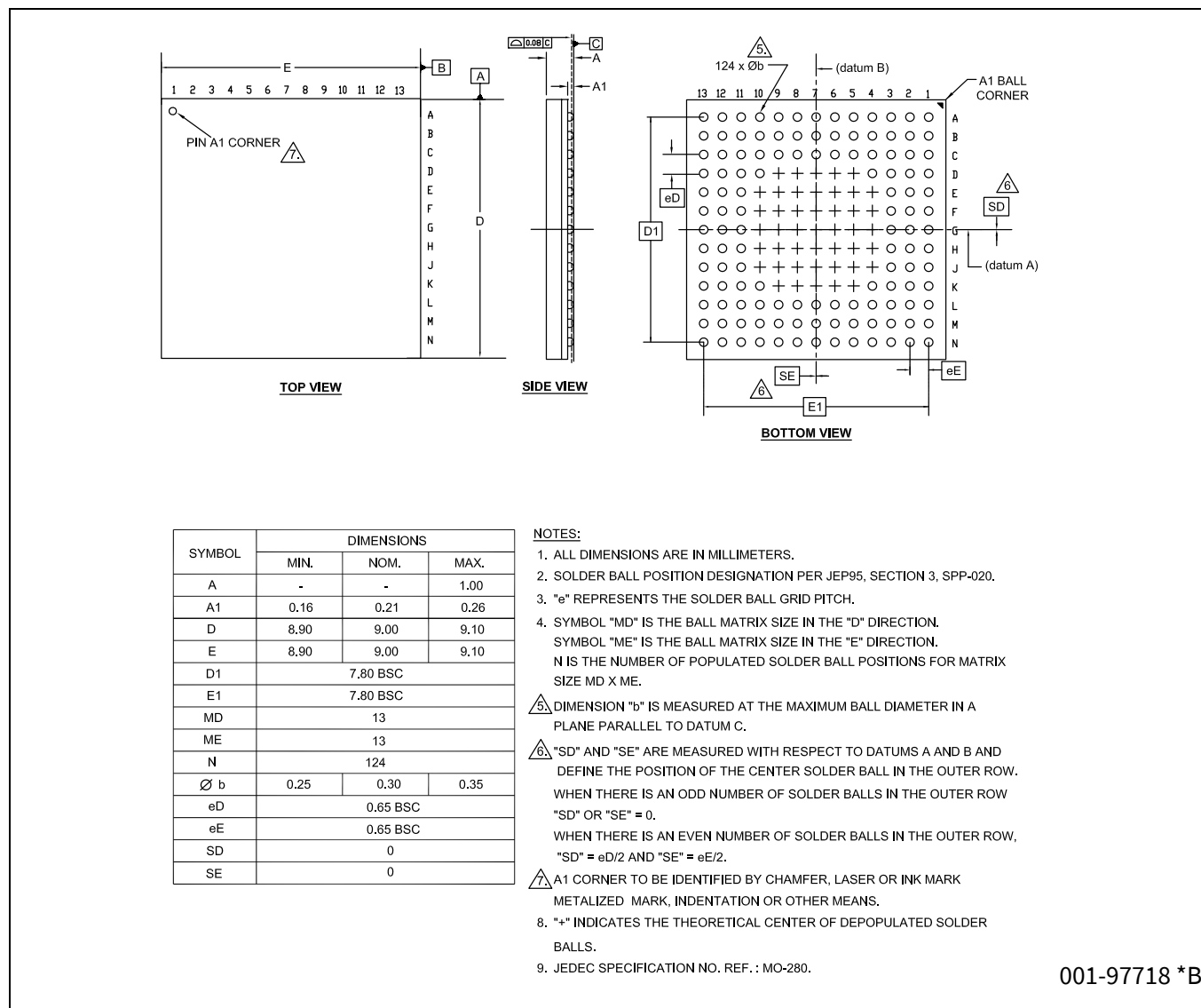
Figure 8 Package outline, 124-ball VFBGA 9.0 × 9.0 × 1.0 mm BZ0AA/VZC124/D2A124 (PG-VFBGA-124)
