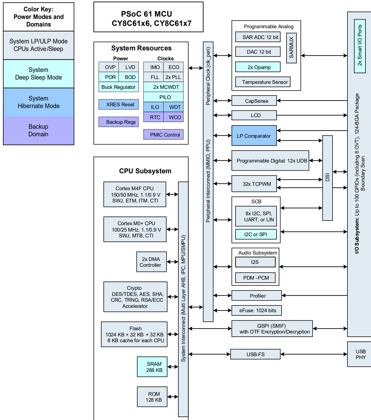
Figure 3. Block Diagram
