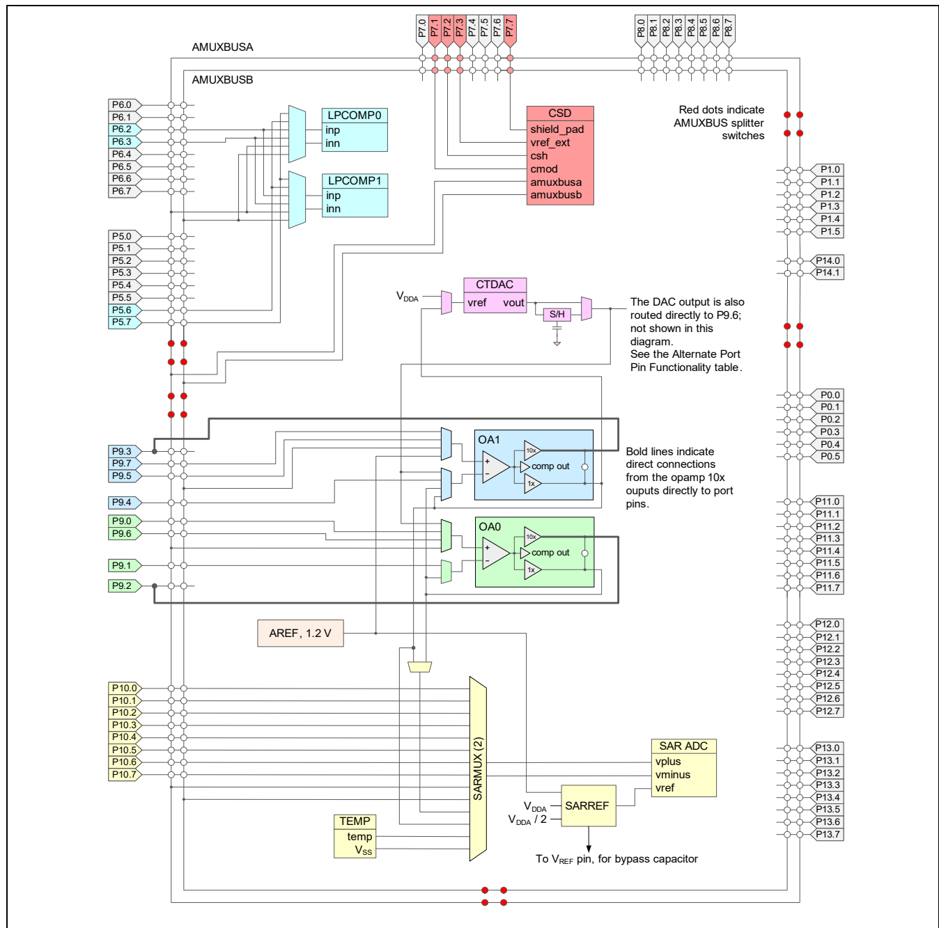
Figure 7 Analog subsystem
