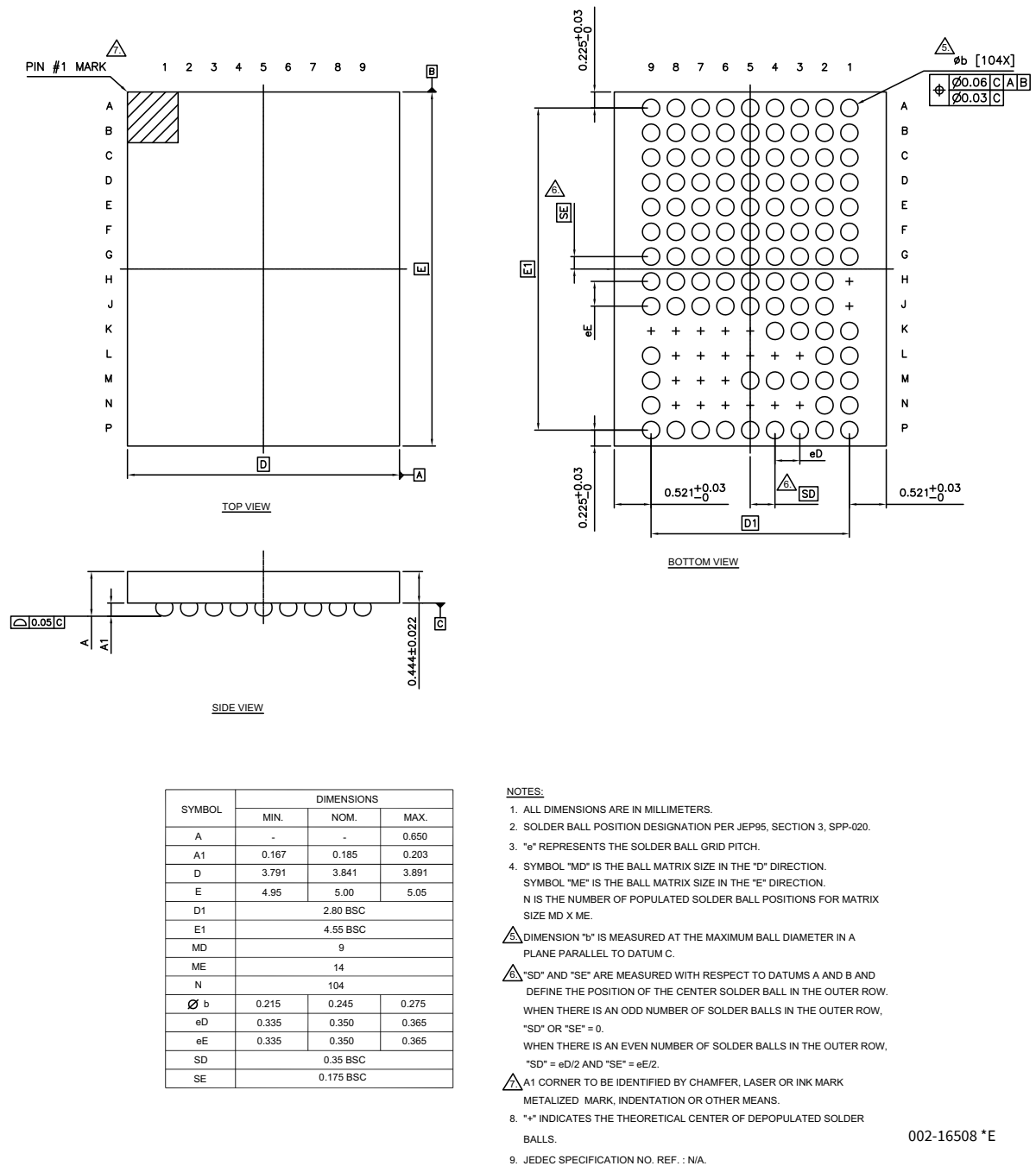
Figure 21 104-M-CSP 3.8 × 5.0 × 0.65 mm
