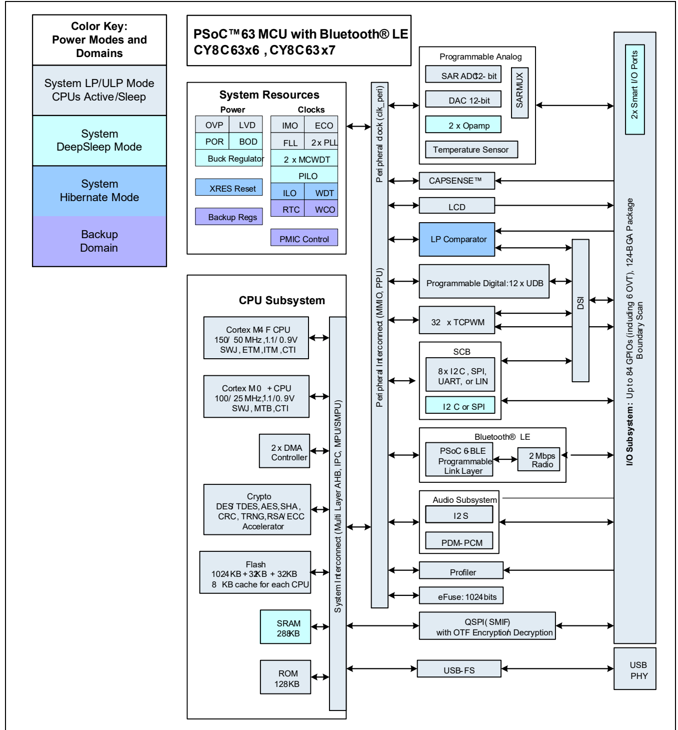
Figure 3 Block diagram
