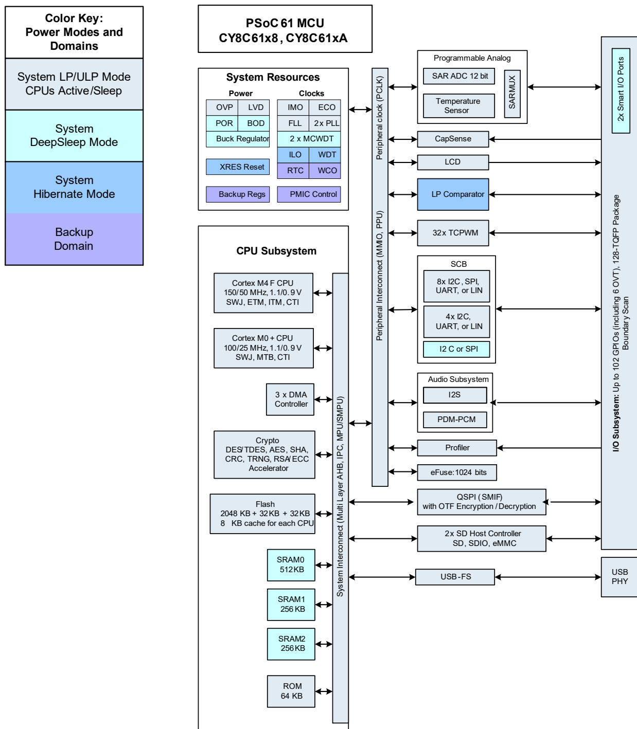
Figure 2. Block Diagram
