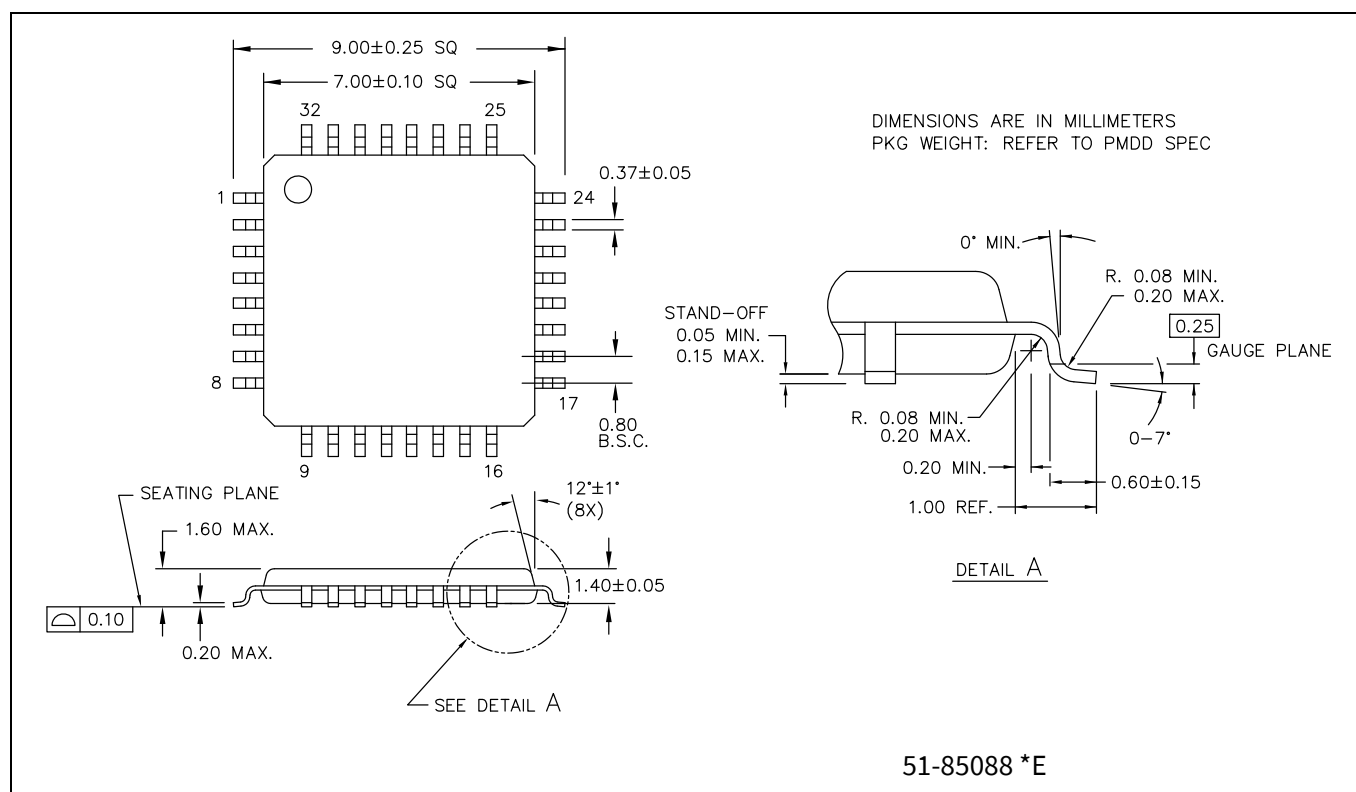
Figure 10 32-pin TQFP (7 × 7 × 1.4 mm) package outline, 51-85088
