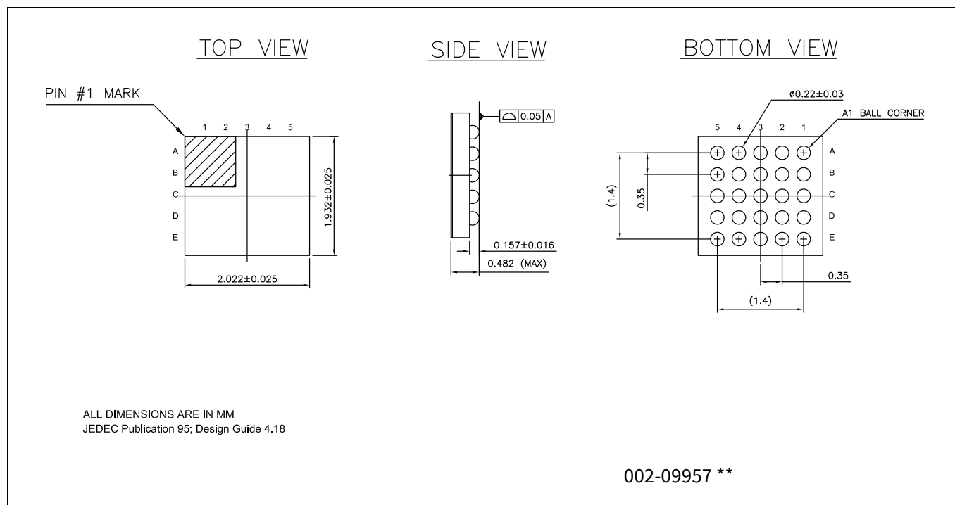
Figure 11 25-ball WLCSP ( 2.02 \times 1.93 \times 0.48 mm) package outline, 002-09957
