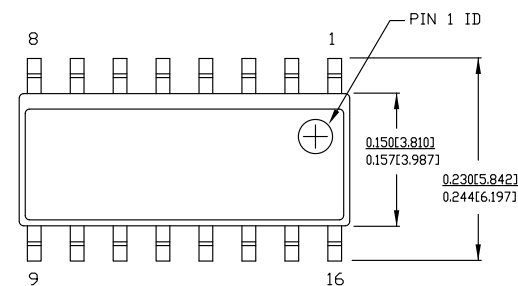
Figure 14. 16-pin (150-mil) SOIC Package Outline
