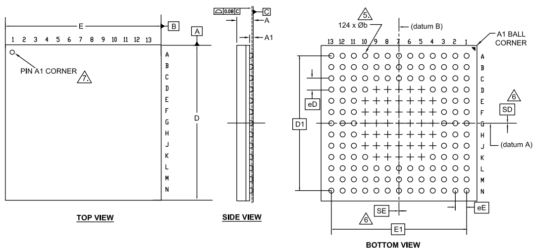
Figure 20. 124-BGA 9.0 × 9.0 × 1.0 mm
