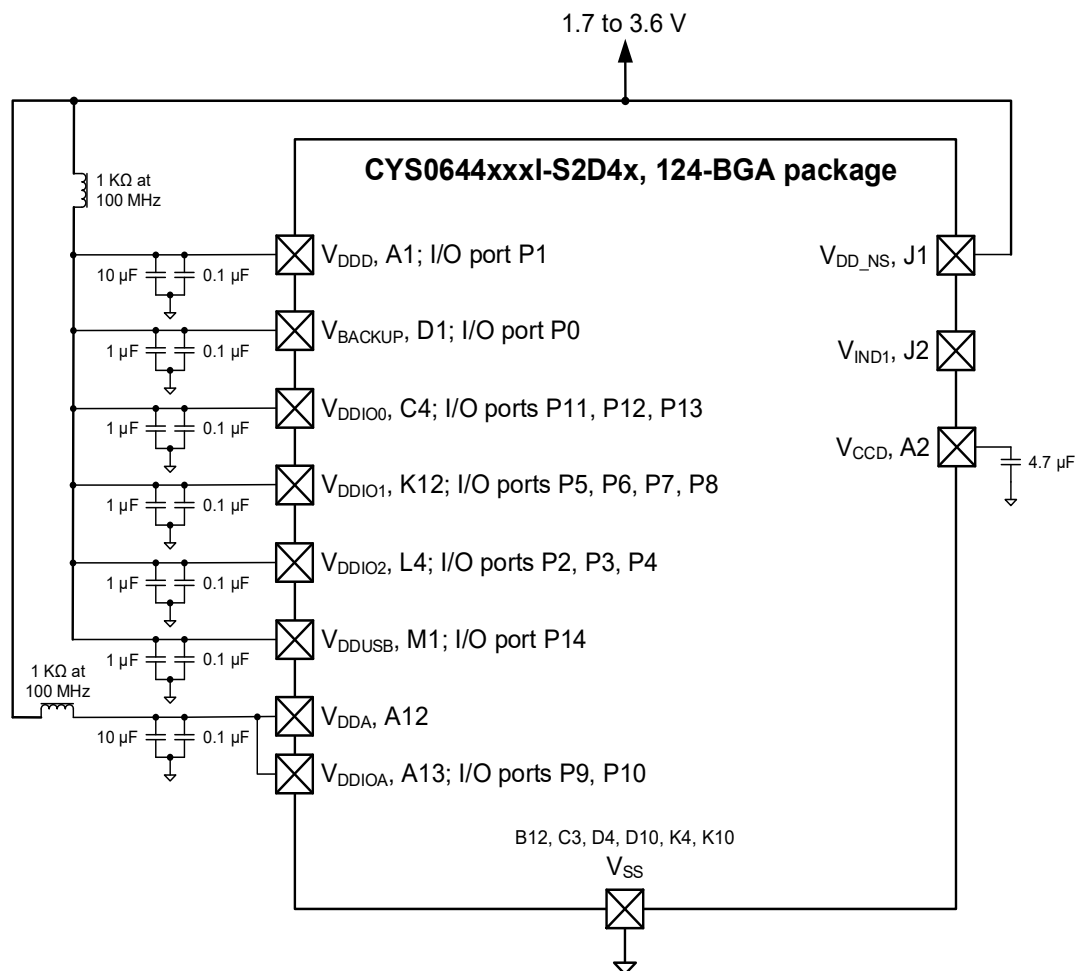
Figure 15. 124-BGA (No Buck) Power Connection Diagram
