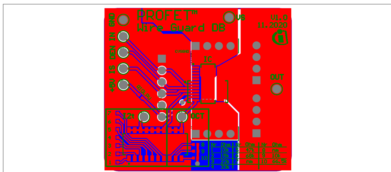
Figure 23 PROFET™ Wire Guard 12V PCB design
