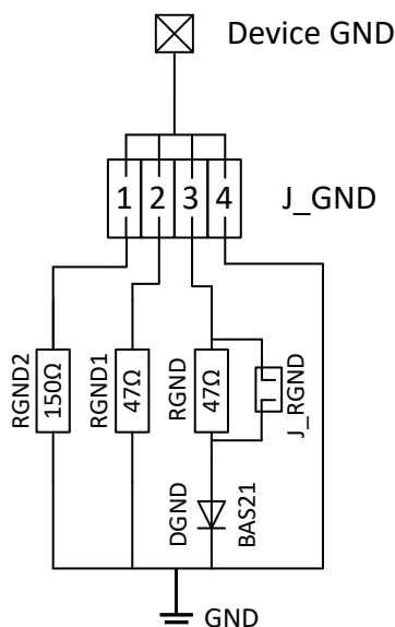
Figure 9 Motherboard V3 GND schematic
