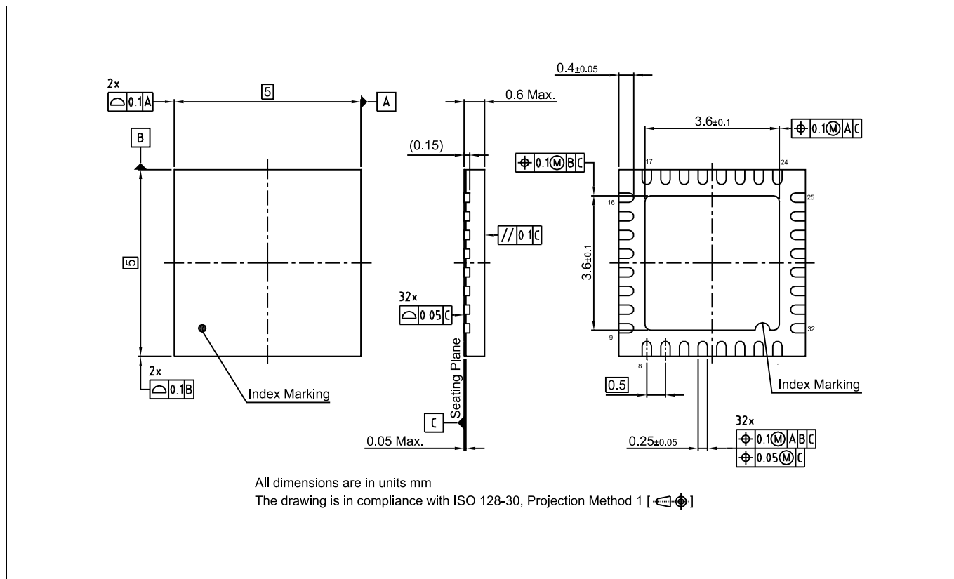
Figure 4 Package dimensions PG-UQFN-32-1,-2
