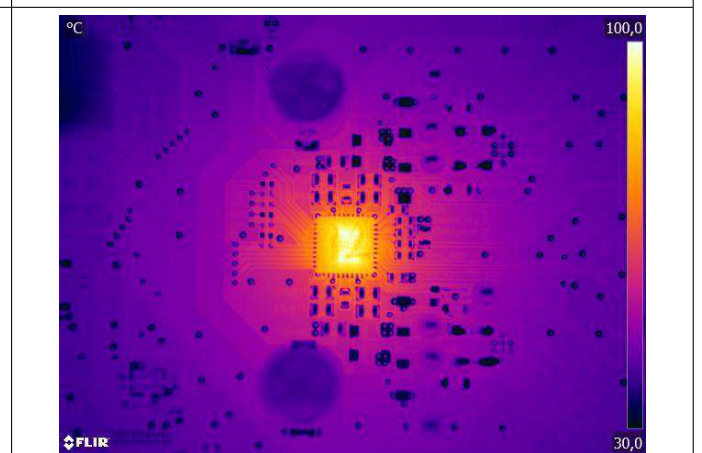
Figure 13.15: Thermal photo of EVAL_AUDIO_MA2304PNS EVK at 2x12 W, 4 \Omega
