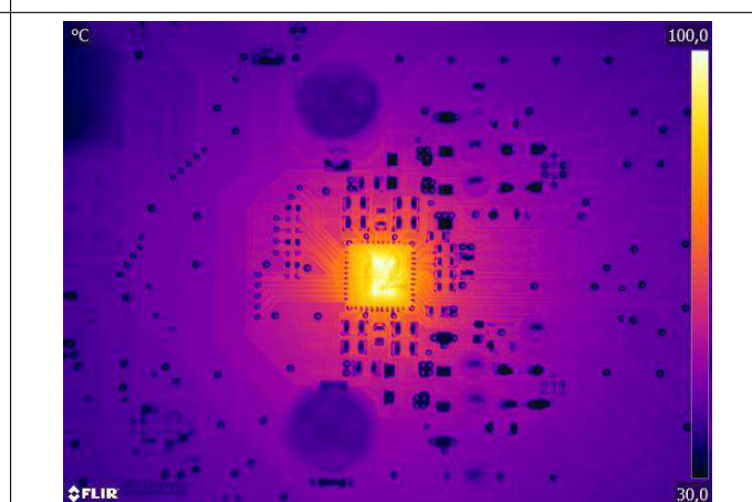
Figure 13.15: Thermal photo of EVAL_AUDIO_MA2304DNS EVK at 2x12 W, 4 \Omega
